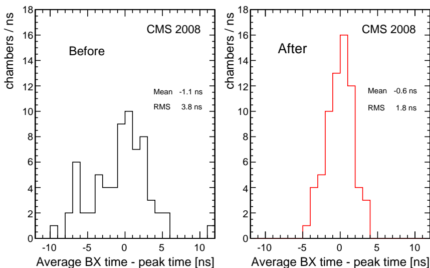
Figure 6. Distribution of the average BX time with respect to the time of the BX bin with the largest number of entries before (left plot) and after (right plot) the delay adjustment for all chambers of sectors 3, 4, 5, 9, 10 and 11 of the wheels 0, 1 and 2. In these data, sector 9 of wheel +2 was not read out.
