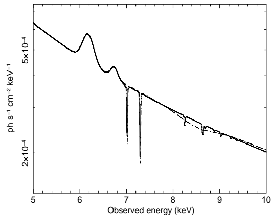
Fig. 4.— Comparison of the best fit model for 3C 120b including the baseline model (see Table 2) plus the Gaussian absorption lines listed in Table 3 (dashed line) or the detailed photo-ionization modeling of the absorber reported in Table 4 (solid line).
