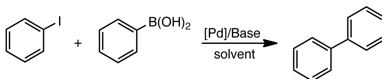
Fig. 6- Suzuki reaction between iodobenzene and phenylboronic acid
