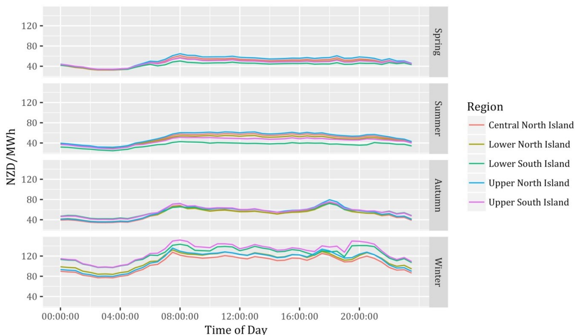
Fig. 16| Average spot market prices
