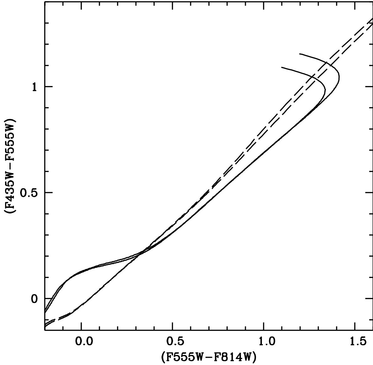
Fig. 11.— (F435W-F555W) vs (F555W-F814W) diagram in the ACS photometric system, for the 0.61 and 1.0 M_{\odot} cooling tracks (including phase separation) with H- (solid lines) and He-atmospheres (dashed lines).
