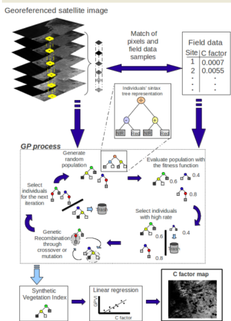
Fig. 1A General flowchart of the methodology to estimate C from vegetation indices synthesized by GP. The figure also shows the syntax tree representation for one of the indices
