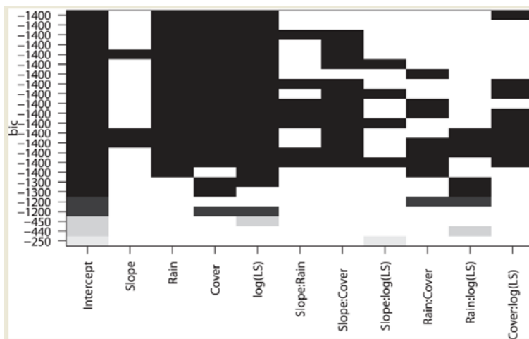
Fig. 7 BIC of the different models obtained by all-subset regression (“:” indicating interaction between the covariates)
