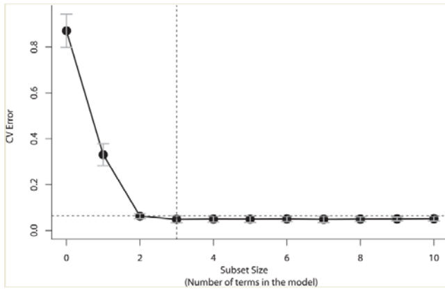
Fig. 8 Model selection with the one-standard deviation rule. (CV = cross-validation)
