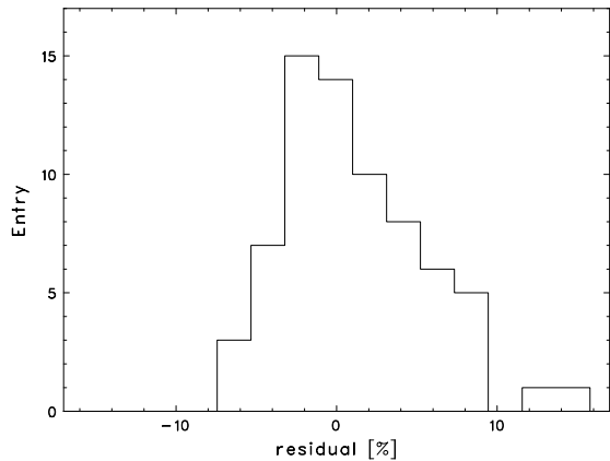
FIG. 5.— The histogram of the fractional residuals between the observed LAT data and the Galactic diffuse model fixed at the best-fit parameters determined by glike . The fluxes of all sources included in the fit-model except for the Galactic diffuse component are subtracted from the observed data. The residual was calculated in 5 energy bands (0.20–0.32 GeV, 0.32–0.50 GeV, 0.50–0.80 GeV, 0.80–1.3, 1.3–10 GeV) for each region as shown in Figure 3.
