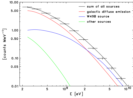
FIG. 7.— The count spectrum within a radius of 0.5 around the W49B source location at (\alpha, \delta) = (287.756, 9.096) . The blue, red, green and black line shows best-fit model curves for the W49B source, the Galactic diffuse emission model, the sum of the other sources (all sources except for the W49B source and the Galactic diffuse model) and the sum of all sources included in the fit-model, respectively.
