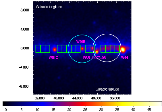
FIG. 3.— The LAT count map above 1 GeV around SNR W49B in units of counts per pixel. The pixel size is 0.^\circ 1 , and Gaussian smoothing is applied with a kernel size of \sigma = 0.^\circ 3 . The W49B source, which is located at the center, is clearly visible. The green boxes ( 1.^\circ 0 \times 1.^\circ 6 ) represent the regions used for the evaluation of spatial dispersion of the difference between the Galactic diffuse model and the observed distribution. The cyan and white circles represent the regions where the flux of the Galactic diffuse model was varied to evaluate effects of spatial dispersion of the model.
