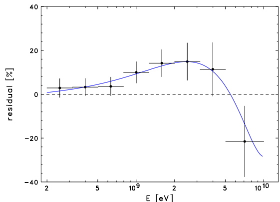
FIG. 4.— The fractional residuals at 8 energy bins in 0.2 to 10 GeV between the observed LAT data and the best-fit Galactic diffuse emission model in the nearby circle centered at (\alpha, \delta)=(288.^\circ 4, 10.^\circ 2) with radius of 0.^\circ 5 . The fluxes of all sources included in the fit-model except for the Galactic diffuse component are subtracted from the observed data. The blue line shows a cubic function fitted to the residual data.
