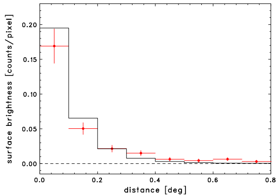
FIG. 2.— The radial profile of the LAT count map with front data in 2 to 30 GeV in units of counts per pixel. The pixel size is 0.^\circ 01 . The origin of the profile is the LAT localization of the W49B source at (\alpha, \delta)=(287.^\circ 756, 9.^\circ 096) . The histogram shows the profile of the effective LAT PSF.
