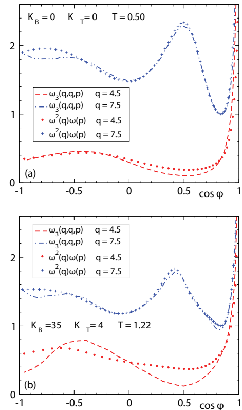
FIG. 10. Comparison of \omega_3(q, q, p = q\sqrt{2(1 - \cos \phi)}) (lines) with the convolution approximation \omega^2(q)\omega(p) (symbols), for two selected values q=4.5 and 7.5 . Panel (a): fully flexible chains at T=0.50 . Panel (b): Stiffest investigated chains at T=1.22 .
