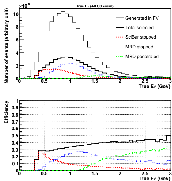
FIG. 8. (color online). (Top) Number of CC events in the SciBar FV as a function of true E_\nu , predicted by the NEUT based simulation. The number of selected events in each sub-sample are also shown. (Bottom) Detection efficiency as a function of true neutrino energy for each sub-sample.
