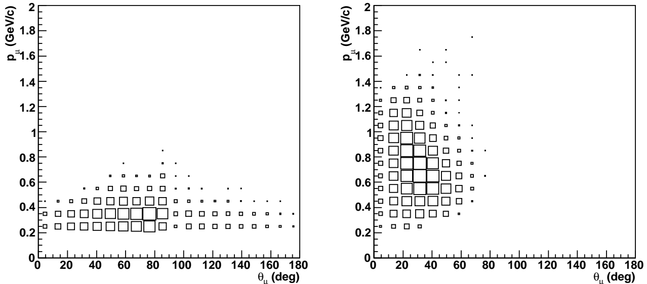
FIG. 10. Data distributions of p_\mu vs. \theta_\mu for the SciBar-stopped (left) and MRD-stopped (right) samples. The size of boxes is proportional to the number of entries.
