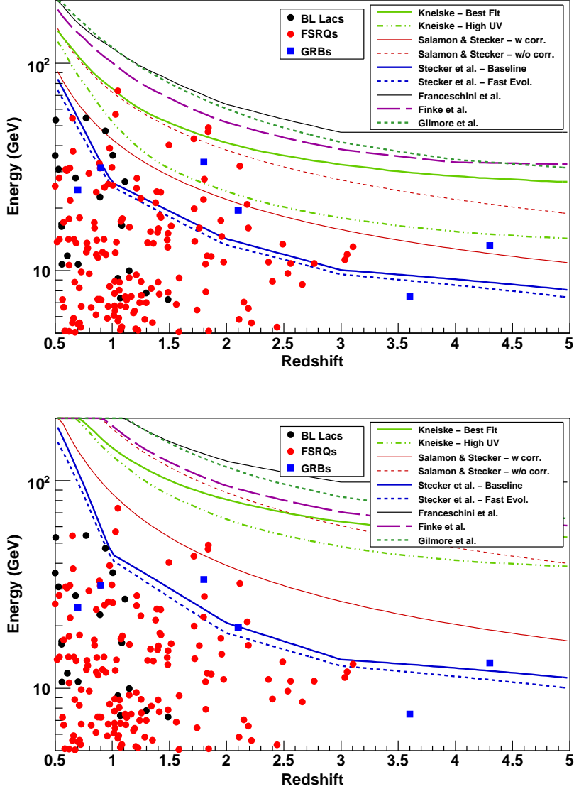
Fig. 3.— Highest-energy photons from blazars and GRBs from different redshifts. Predictions of \gamma\gamma optical depth \tau_{\gamma\gamma} = 1 (top panel) and \tau_{\gamma\gamma} = 3 (bottom panel) from various EBL models are indicated by lines. Photons above model predictions in this figure traverse an EBL medium with a high \gamma -ray opacity. The likelihood of detecting such photon considering the spectral characteristics of the source are considered in the method presented in section 3.2.1.
