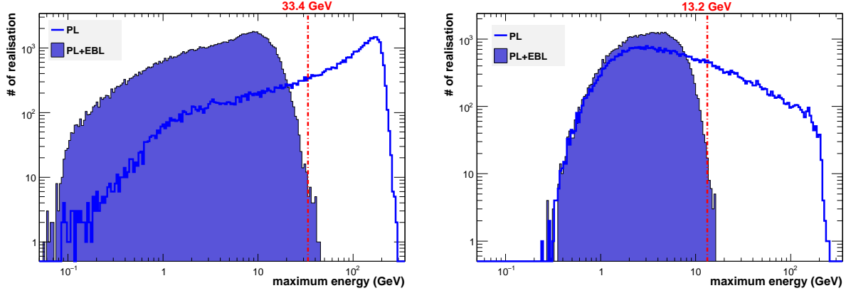
Fig. 5.— Distributions of the highest energy photons from simulations performed with estimates of our intrinsic spectra for GRB 080916C (left panel) and GRB 090902B (right panel), folded with EBL attenuation calculated using the Stecker et al. (2006) baseline model. The total number of realizations ( 10^5 ) in both the power-law and power-law convolved with the EBL cases is the same.
