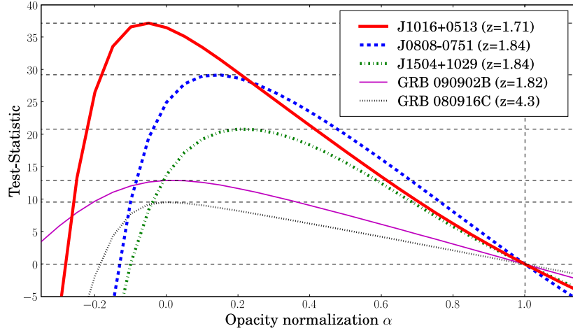
Fig. 6.— Test statistic (TS) as a function of the \gamma -ray optical depth normalization parameter calculated from the likelihood ratio test (LRT) for J1016+0513, J0808-0751, J1504+1029 and GRBs 090902B and 080916C. The "baseline" model of Stecker et al. (2006) has been used and the rejection for this model can be directly read out as \Delta TS between \alpha = 1 and the best fit \alpha for the source (horizontal dashed line). The confidence interval for the normalization parameter can be obtained using \Delta TS = CL^2 where CL is the confidence level.
