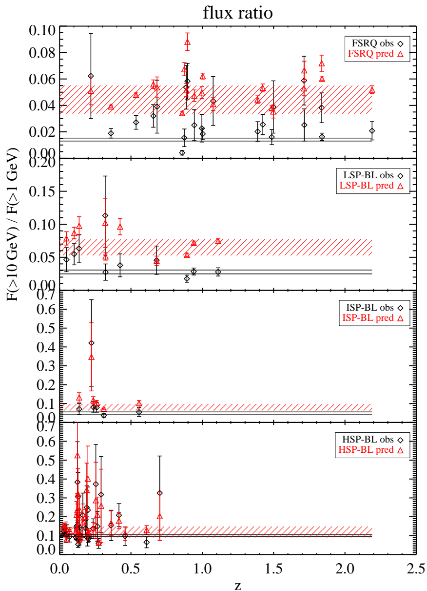
Fig. 2.— Flux ratio F(\geq 10 \text{ GeV})/F(\geq 1 \text{ GeV}) as a function of redshift, in the Fermi LAT energy range, for FSRQs and BL Lac populations. The black diamonds are the observed ratios, while the red triangles show the ratio expected assuming an unbroken power law and no EBL attenuation. The black horizontal solid lines and red cross-hatched regions correspond to the mean observed ratios and expected ratios with errors.
