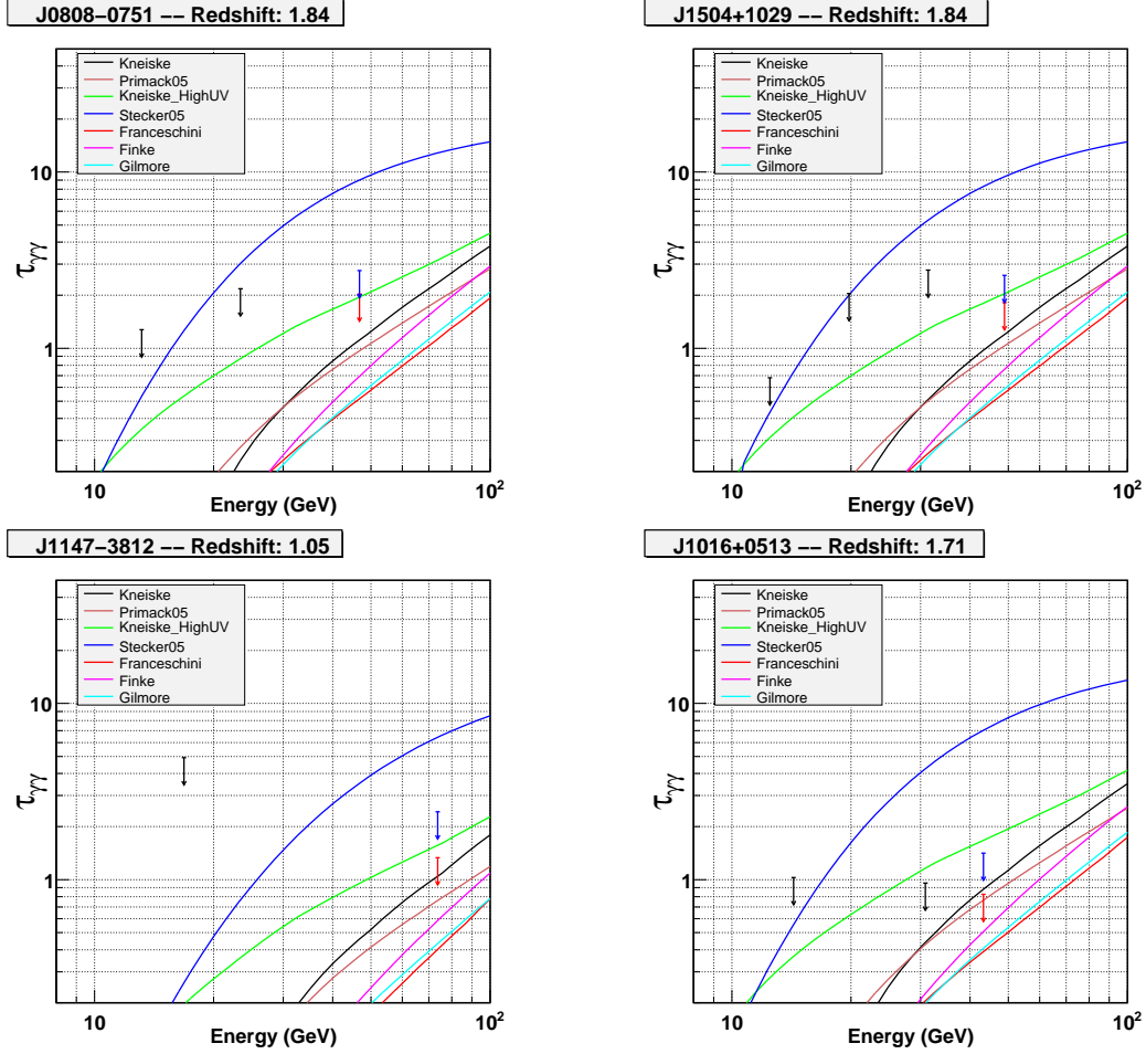
Fig. 7.— Derived upper limits for the optical depth of \gamma -rays emitted at z=1.84 (J0808-0751, J1504+1029), z=1.05 (J1147-3812) and z=1.71 (J1016+0513). Black arrows: upper limits at 95% c.l. in all energy bins used to determine the observed flux above 10 GeV. Red arrow: upper limits at 95% c.l. for the highest energy photon. Blue arrow: upper limit at 99% c.l. for the highest energy photon. The upper limits are inconsistent with the EBL models that predict the strongest opacity.
