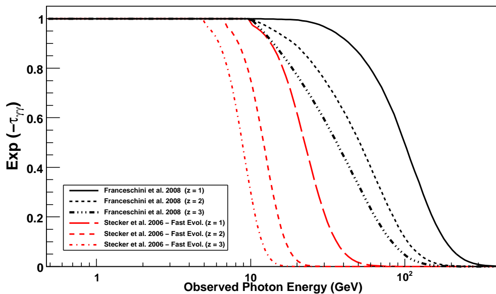
Fig. 1.— Attenuation as a function of observed gamma-ray energy for the EBL models of (Franceschini et al. 2008) and (Stecker et al. 2006). These models predict the minimum and maximum absorption of all models in the literature, and thus illustrate the range of optical depths predicted in the Fermi -LAT energy range.
