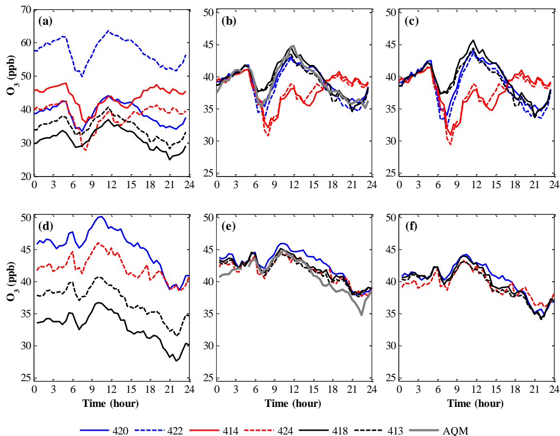
Figure 1. Daily patterns of 30 min. average O_3 concentrations during weekdays (Sunday to Thursday; upper row) and Saturdays (lower row) (a,d) before calibration; (b,e) after calibration against a nearby AQM measurements from 1:00 to 4:00 am; (c,f) and after calibration against the mean half-hourly reading between 1:00 and 4:00 am of all the WDESN nodes. (Reproduced with permission from [19]).
