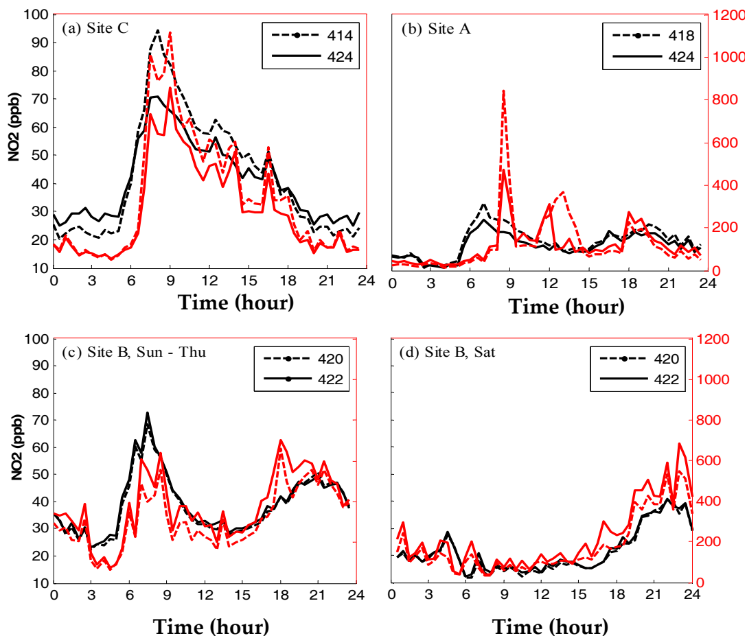
Figure 2. Daily patterns of 30 min average NO 2 (black) and total volatile organic compounds (TVOC) (red) concentrations in (a) site C during weekdays (Sunday to Thursday); (b) site A during weekdays (note the adaptation of node 424 to its microenvironments upon relocation); (c) site B during weekdays; and (d) site B during Saturdays. The MSUs were deployed in a residential neighborhood after they were calibrated while collocated at an AQM station within the neighborhood. (Reproduced with permission from [19]).
