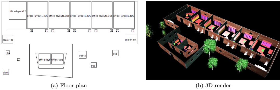
Fig. 9: An output of the Virtual World Grammar using shape grammar 1
