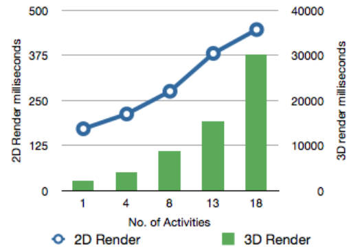
Fig. 6: Performance measurements of VWG
