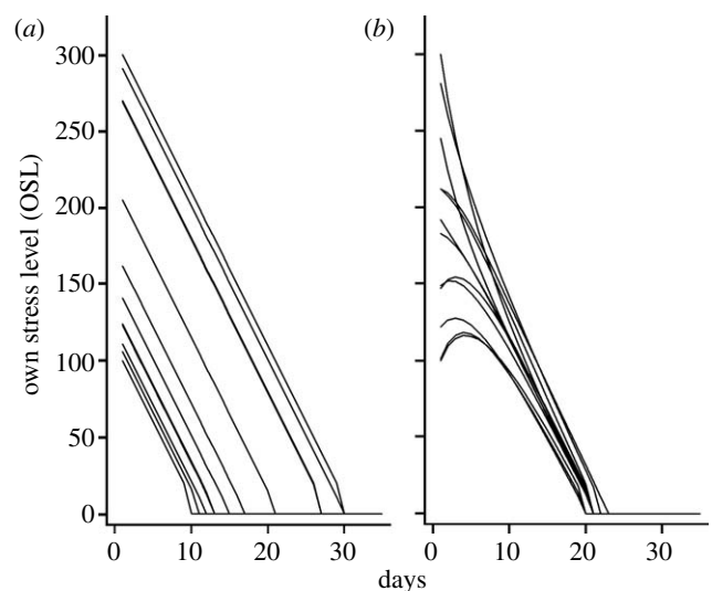
Figure 1. Individual stress-level (OSL) dynamics. (a) No neighbour interaction (neighbourhood relevance NR=0); (b) NR=0.2. The upper and lower curves present the dynamics of the individual with the highest (300) and lowest (100) initial stress levels, respectively. The other 10 trajectories shown are from randomly selected birds. Note that when females achieve a stress level of 10 or less they start incubating (at the end of each individual trajectory), and thus the stress level becomes 0 the following day.
