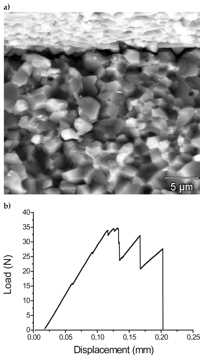
Figure 1. Alumina-aluminium titanate laminate fabricated using a combination of tape casting, dipping and EPD 12 .
