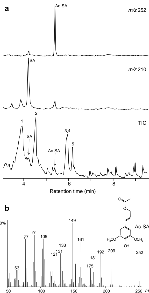
Fig. 7. GC-MS analysis of the M. textilis extracts. (a) Expanded region of the total-ion chromatogram (TIC) from the acetone extract of the whole fiber showing the presence of sinapyl acetate (Ac-SA) and free sinapyl alcohol (SA) peaks together with other extractives (1, p -coumaric acid; 2, palmitic acid; 3, linoleic acid; 4, oleic acid; and 5, stearic acid); and reconstructed chromatograms based on selected ions, m/z 252 and m/z 210, enabling localization of the Ac-SA and SA peaks, respectively. (b) Mass spectrum of the Ac-SA peak enabling its identification as \gamma -acetylated sinapyl alcohol.
