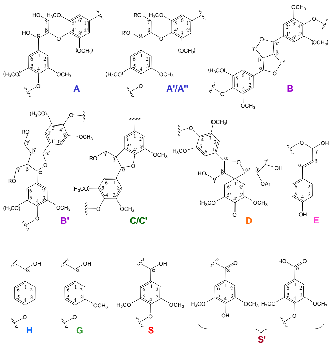
Fig. 5. Main classical and acylated substructures, involving different side-chain linkages, and aromatic units identified by 2D NMR of the A. sisalana , M. textilis and C. sativa lignins: (A) \beta -O-4' substructure; (A') \gamma -acylated \beta -O-4' substructure ( R , acetyl/ p -coumaroyl; R' , H); (A'') \alpha -acylated \beta -O-4' substructure, being especially abundant in the in vitro acetylated lignins where it is diacylated ( R , acetyl/ p -coumaroyl; and R' , acetyl); (B) resinol substructure, formed by \beta - \beta' coupling and \alpha -O- \gamma' and \gamma -O- \alpha' bonding during quinone methide rearomatization; (B') di- \gamma -acylated mono-tetrahydrofuran structure formed by \beta - \beta' coupling and subsequent \alpha -O- \alpha' bonding ( R , acetyl/ p -coumaroyl); (C) phenylcoumaran, formed by \beta -5' coupling and subsequent \alpha -O-4' bonding ( R , H); (C') \gamma -acylated phenylcoumaran ( R , acetyl); (D) Spirodienone, formed by \beta -1' coupling and subsequent \alpha -O- \alpha' bonding; (H) p -hydroxyphenyl unit; (G) guaiacyl unit; (S) syringyl unit; and (S') oxidized syringyl units with a C_x ketone or a C_x carboxyl group. A–D correspond to non-acylated substructures; A' and B' correspond to naturally-acylated substructures; and A'' and C' basically correspond to in vitro acetylated substructures. No specific signals corresponding to acylated D could be detected (even after in vitro acetylation). Only main substructures (with a relative abundance >1% of total side-chains) are presented.
