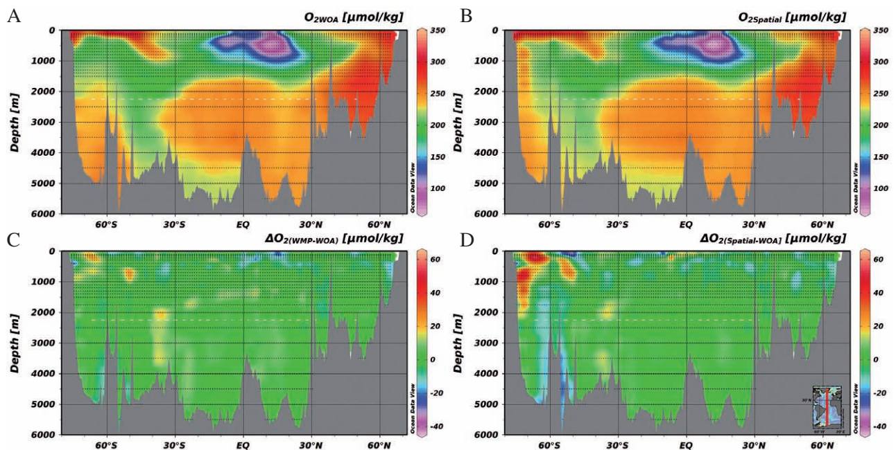
FIG. 5. – \text{O}_2 ( \mu\text{mol kg}^{-1} ) variability along 28^\circ\text{W} from the WOA05 dataset (A), spatially interpolated from CARINA data (B). Residuals of WMP interpolated (C) and spatially interpolated (D) \text{O}_2 , both as interpolated minus WOA05.
