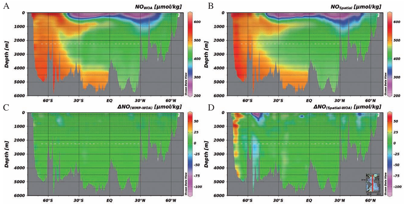
FIG. 4. – NO ( \mu\text{mol kg}^{-1} ) variability along 28^\circ\text{W} from the WOA05 dataset (A), spatially interpolated from CARINA data (B). Residuals of WMP interpolated (C) and spatially interpolated (D) NO, both as interpolated minus WOA05.
