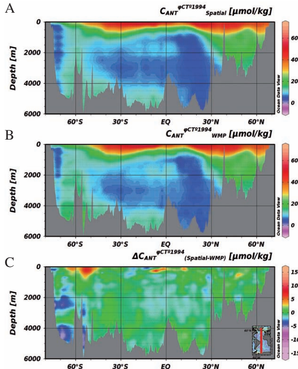
FIG. 6. – C_{ANT} ( \mu\text{mol kg}^{-1} ) determined by the \phi C_T^{\circ} method along 28°W using spatial interpolation (A) and WMP interpolation (B). Residuals between the two interpolations are shown (C) as spatially interpolated minus WMP interpolated.
