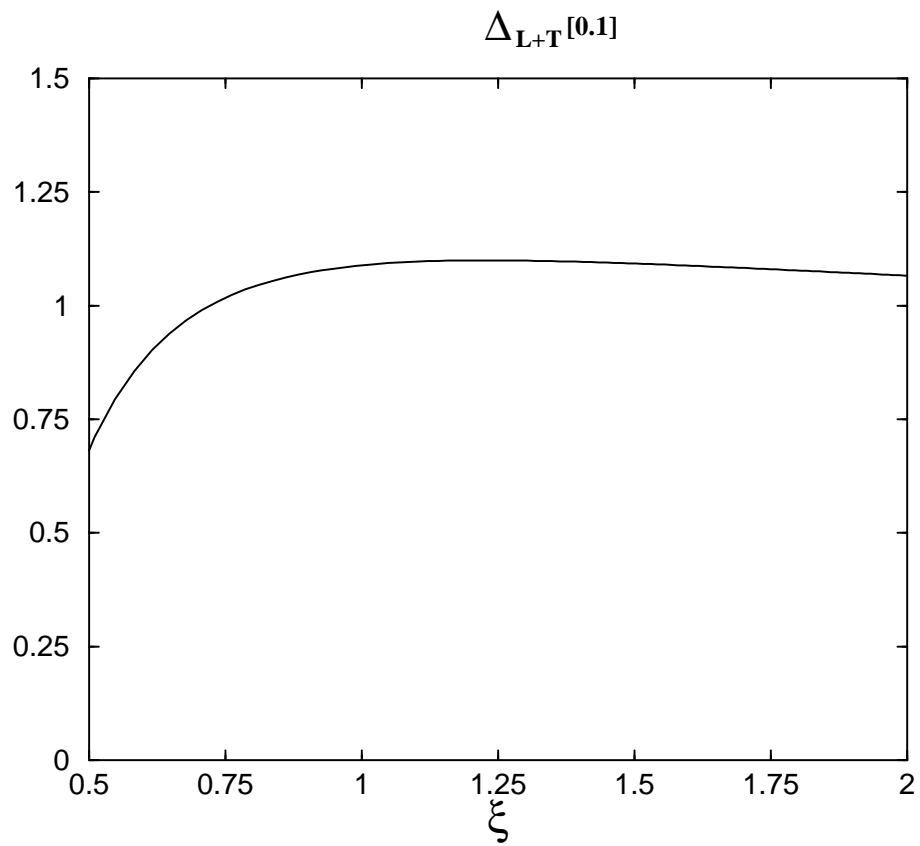
Figure 1: Variation of \Delta_{L+T}[0.1] with the renormalization-scale factor \xi , to four loops.
