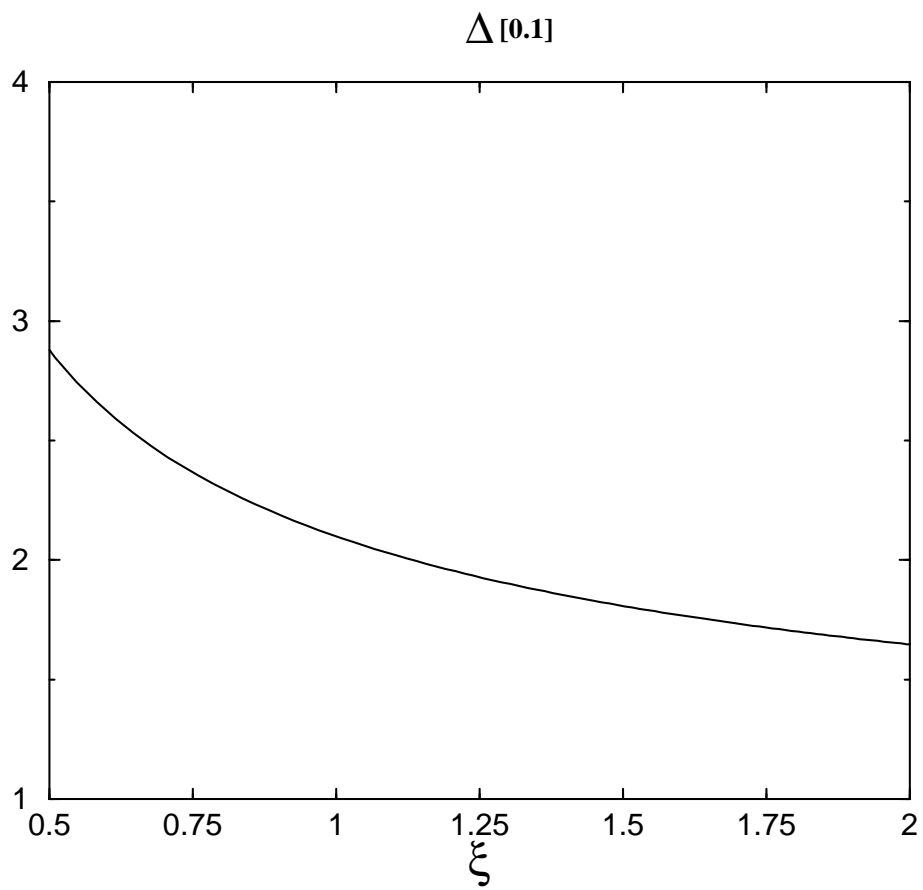
Figure 3: Variation of \Delta[0.1] with the renormalization-scale factor \xi , to four loops.
