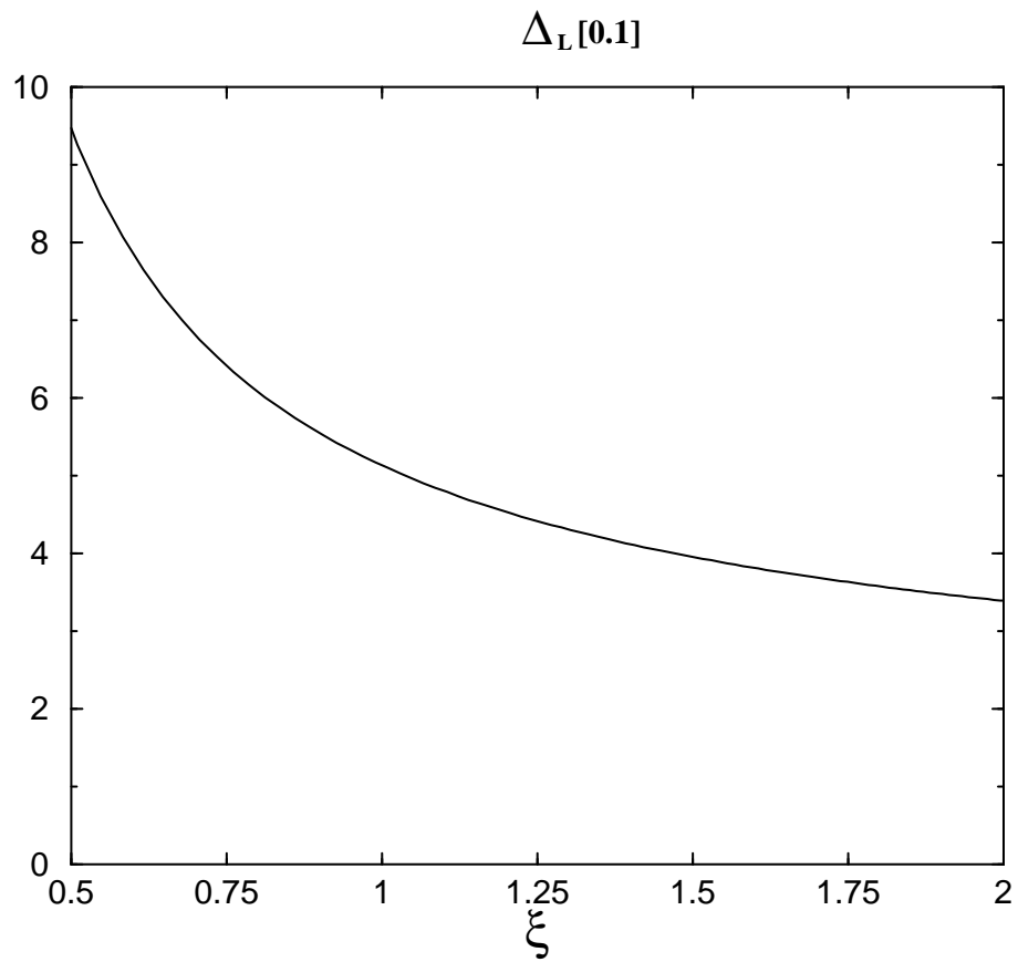
Figure 2: Variation of \Delta_L[0.1] with the renormalization-scale factor \xi , to four loops.
