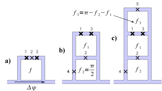
FIG. 1: Schemes for ultrastrong coupling between a qubit and a transmission line. (a) Basic setup of a qubit coupled directly to the line. \Delta\psi is the phase difference between the nodes in which the qubit and line intersect. (b) With a second loop, the coupling can be modulated. (c) A slightly improved setup in which the qubit is better decoupled from the flux f_2 .
