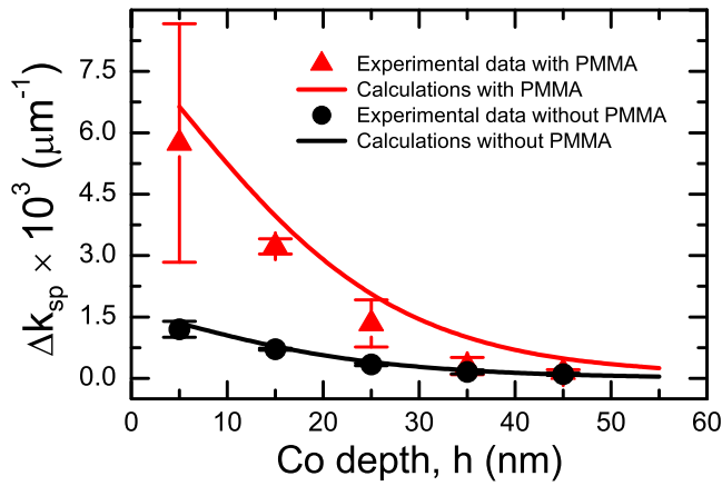
FIG. 2. (Color online) Evolution of the SPP wave vector modulation with the Co layer position for a set of metallic multilayers covered with 60 nm of PMMA and without coverage.
