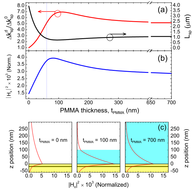
FIG. 3. (Color online) (a) Calculated modulation enhancement (left axis) and SPP propagation distance (right axis) as a function of the thickness of PMMA coverage for an Au/Co/Au trilayer with h=15 nm. (b) Normalized magnetic field intensity calculated at the center of the Co layer. The dashed line marks the thickness value used experimentally, 60 nm. (c) Normalized magnetic field intensity distribution along the vertical direction for three PMMA thicknesses: 0, 100, and 700 nm. The different background colors account for the different materials in the structure.
