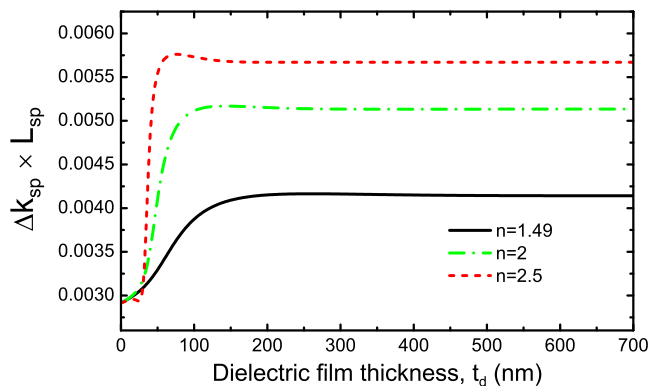
FIG. 4. (Color online) Figure of merit \Delta k_{sp} \times L_{sp} for an Au/Co/Au trilayer with h=15 nm and three different dielectrics.
