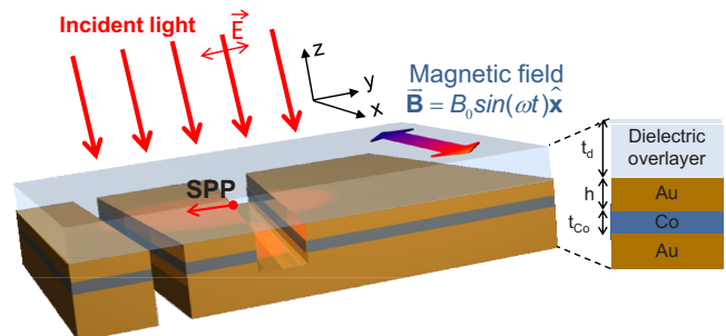
FIG. 1. (Color online) Sketch of the magneto-plasmonic interferometer consisting of a metallic Au/Co/Au trilayer covered by a thin dielectric film.
