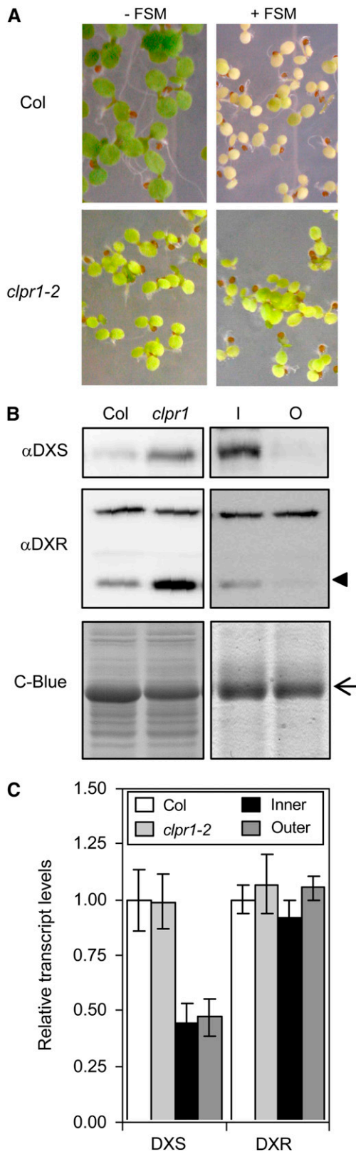
Figure 8. Role of the Plastidial Clp Protease Complex in the Degradation of DXS and DXR.
