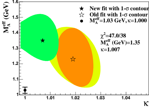
FIG. 9: (Color online). The 1\sigma contour plot for the M_A^{\text{eff}} - \kappa fit. The filled star shows the best fit point and 1\sigma contour extracted from this work. The open star indicates the best fit point and 1\sigma contour from the previous work [11]. Two error ellipses are shown for the previous work, the larger reflects the total uncertainty ultimately included in Ref. [11]. The circle indicates the world-average value for M_A [9].
