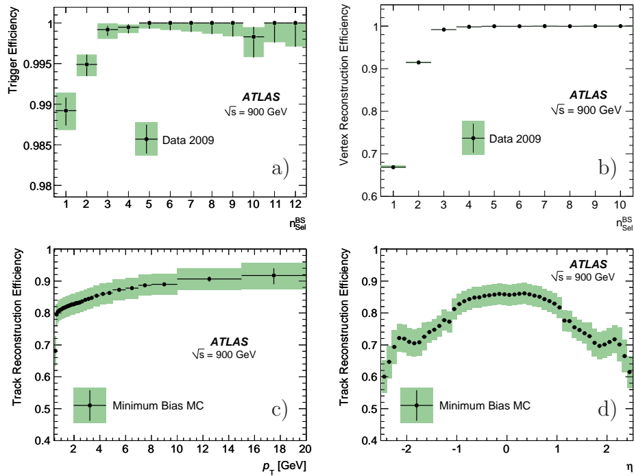
Figure 2: Trigger (a) and vertex-reconstruction (b) efficiencies as a function of the variable n_{\text{Sel}}^{\text{BS}} defined in Section 4; track-reconstruction efficiency as a function of p_T (c) and of \eta (d). The vertical bars represent the statistical uncertainty, while the shaded areas represent the statistical and systematic uncertainties added in quadrature. The two bottom panels were derived from the PYTHIA ATLAS MC09 sample.
