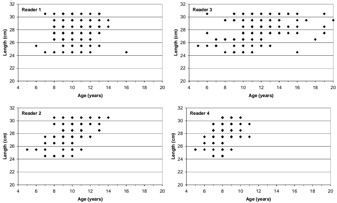
Fig. 7. Age reading scores for otoliths of demersal S. mentella from the East Greenland shelf and pelagic S. mentella from the Irminger Sea combined, illustrating the range and variation of readings and relationship with fish total length.
