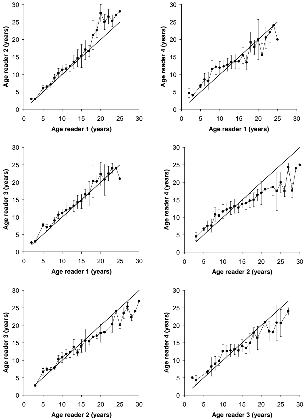
Fig. 1. Age bias plots for the reader comparisons based on the S. marinus otoliths from the Icelandic shelf (see Stransky et al. 2001, adding readings of Partner 2 carried out in 2002, Stransky et al. 2002). Each error bar represents the standard deviation around the mean age assigned by one reader for all fish assigned a given age by the second reader. The 1:1 equivalence (straight line) is also indicated.
