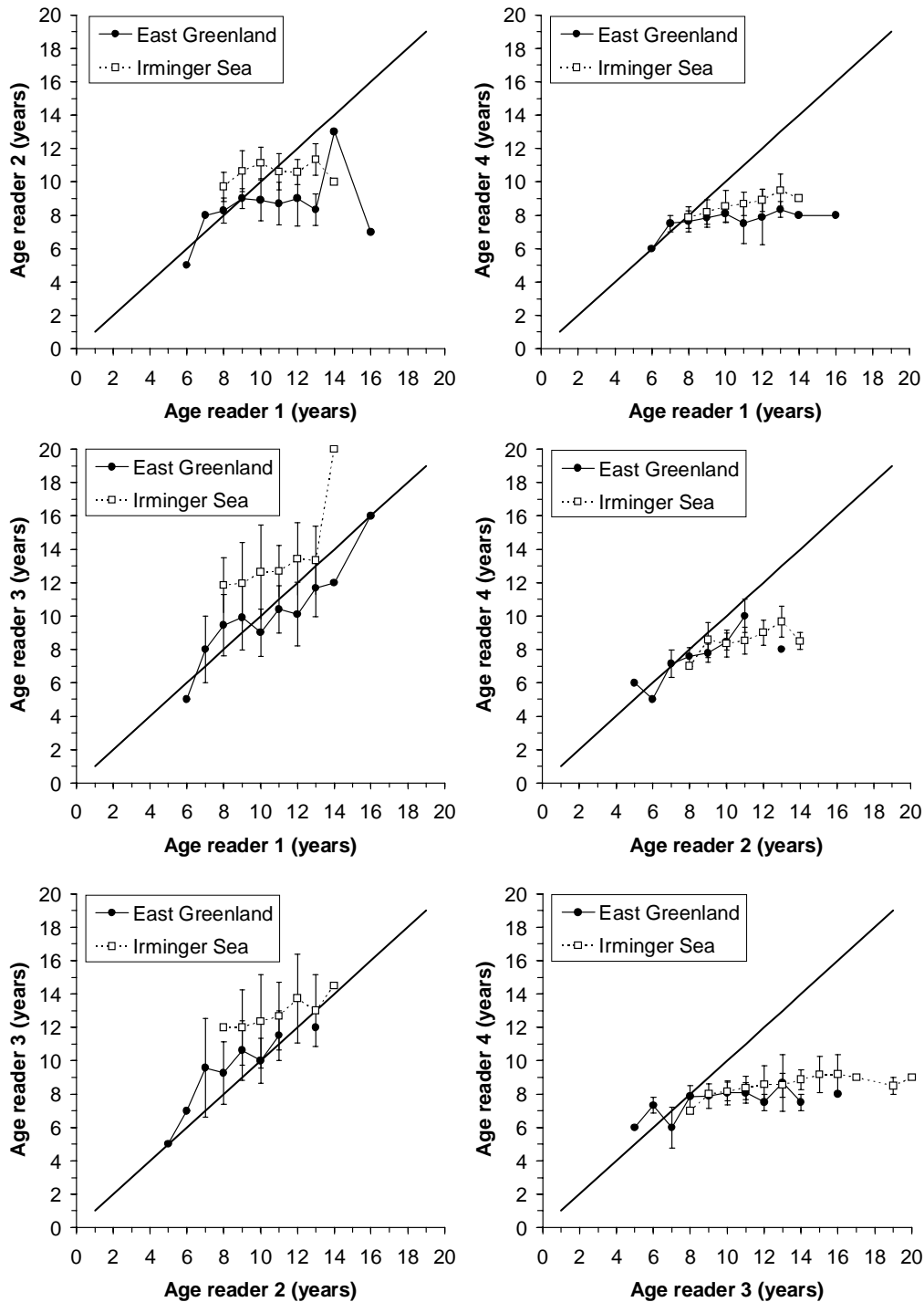
Fig. 5. Age bias plots for the reader comparisons based on otoliths of demersal S. mentella from the East Greenland shelf and pelagic S. mentella from the Irminger Sea. Each error bar represents the standard deviation around the mean age assigned by one reader for all fish assigned a given age by the second reader. The 1:1 equivalence (straight line) is also indicated.
