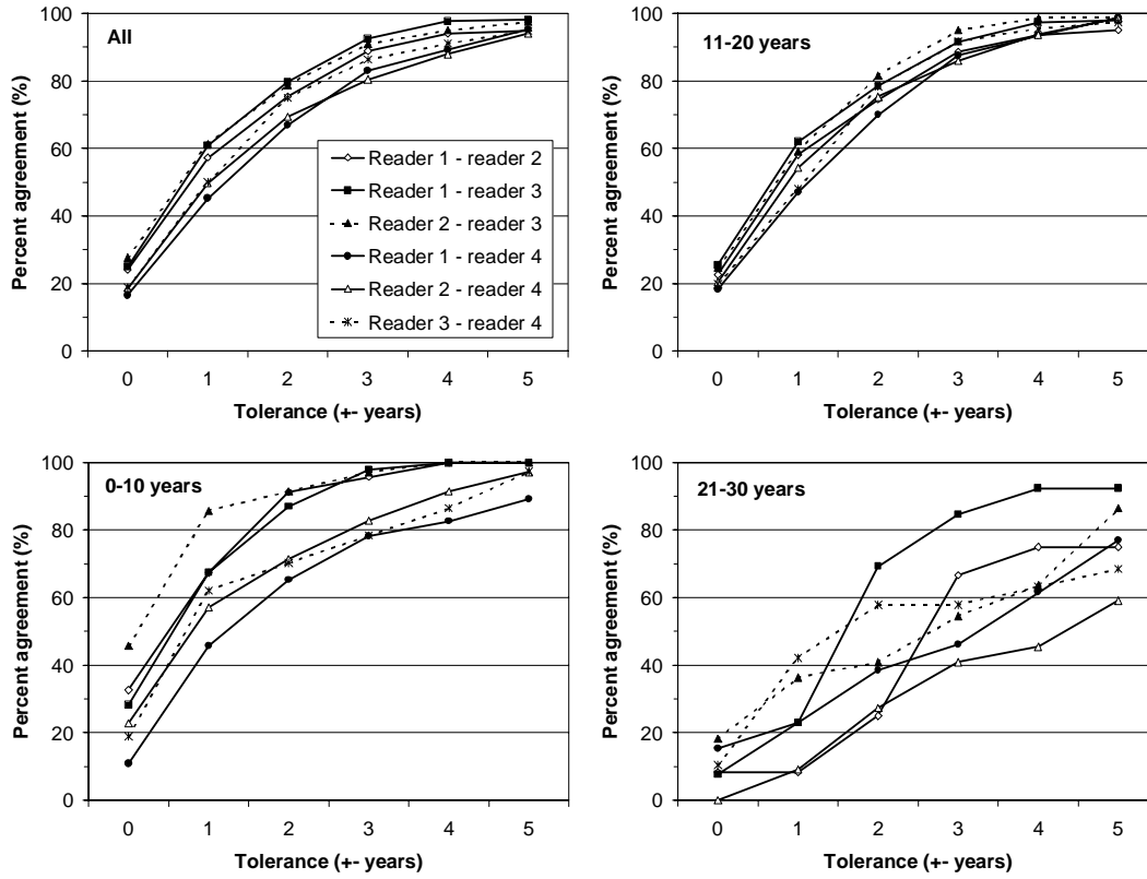
Fig. 2. Percent agreement plots for the reader comparisons based on the S. marinus otoliths from the Icelandic shelf (see Stransky et al. 2001, adding readings of Partner 2 carried out in 2002, Stransky et al. 2002) for a tolerance level (deviation of assigned ages between both readers) of \pm 0 (total agreement) to \pm 5 years. These were applied to all age groups and sub-sets of age ranges assigned by the first reader.
