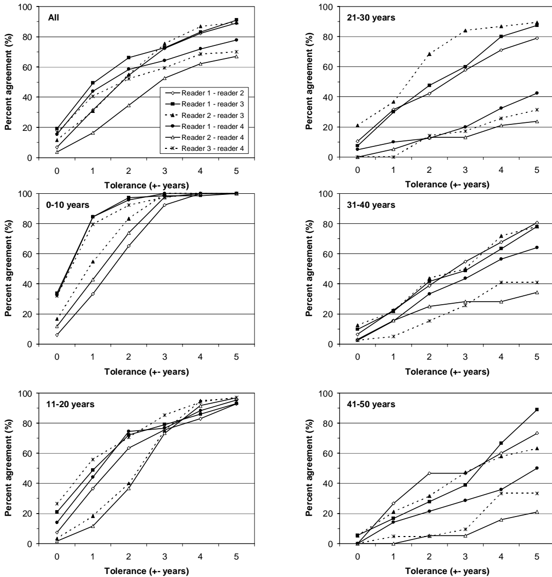
Fig. 4. Percent agreement plots for the reader comparisons based on the pelagic S. mentella otoliths from the Irminger Sea (see Stransky et al. 2001, adding readings of Partner 2 carried out in 2002, Stransky et al. 2002) for a tolerance level (deviation of assigned ages between both readers) of \pm 0 (total agreement) to \pm 5 years. These were applied to all age groups and sub-sets of age ranges assigned by the first reader.
