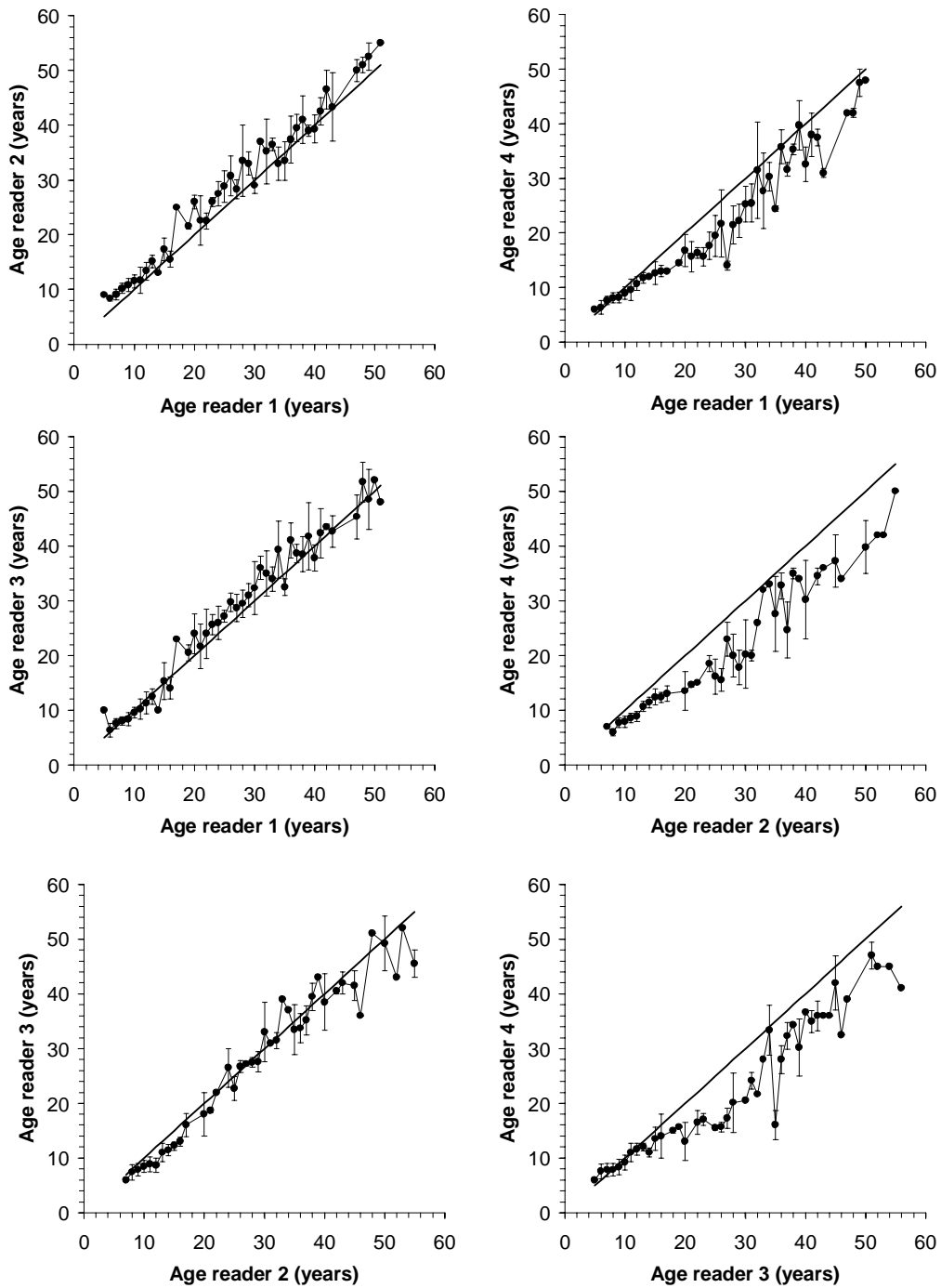
Fig. 3. Age bias plots for the reader comparisons based on the pelagic S. mentella otoliths from the Irminger Sea (see Stransky et al. 2001, adding readings of Partner 2 carried out in 2002, Stransky et al. 2002). Each error bar represents the standard deviation around the mean age assigned by one reader for all fish assigned a given age by the second reader. The 1:1 equivalence (straight line) is also indicated.
