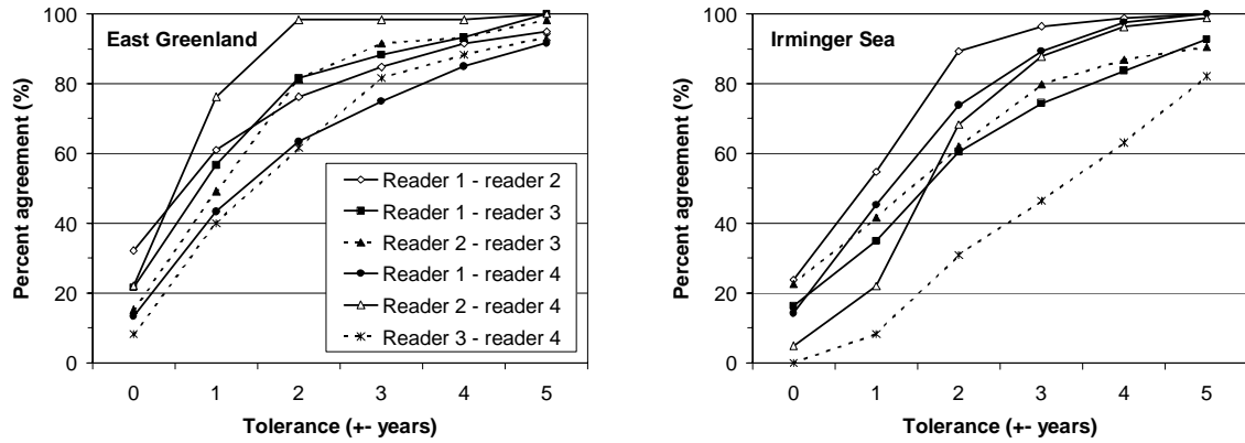
Fig. 6. Percent agreement plots for the reader comparisons based on otoliths of demersal S. mentella from the East Greenland shelf and pelagic S. mentella from the Irminger Sea for a tolerance level (deviation of assigned ages between both readers) of \pm 0 (total agreement) to \pm 5 years. These were applied to all age groups and sub-sets of age ranges assigned by the first reader.
