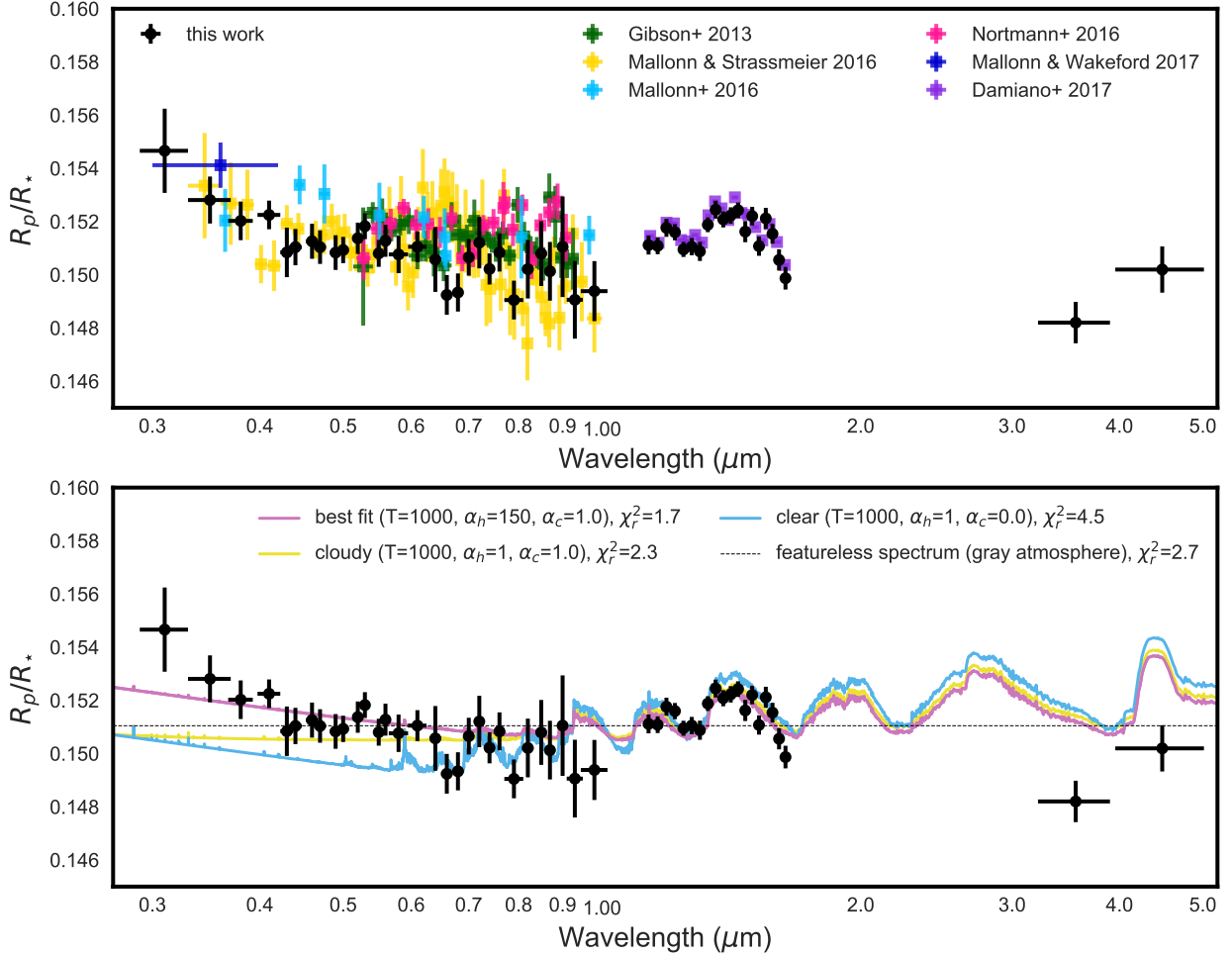
Figure 9. Top: Broadband transmission spectrum for HAT-P-32Ab from HST STIS+WFC3 and Spitzer IRAC (black points). Ground-based measurements from Gibson et al. 2013 (green), Mallonn & Strassmeier 2016 (yellow), Mallonn et al. 2016 (light blue), Nortmann et al. 2016 (pink), Mallonn & Wakeford 2017 (dark blue), and Damiano et al. 2017 (purple) are shown for comparison. Bottom: A subset of the best-fitting theoretical models (lines) fit to the broadband transmission spectrum. The increase in transit depth near 1.4 \mu\text{m} corresponds to a near-infrared \text{H}_2\text{O} bandhead. The average R_p/R_* baseline of the transmission spectrum (dashed black line) is shown for reference.
