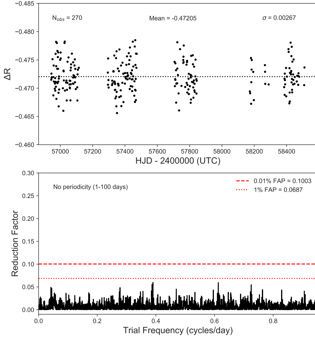
Figure 2. Top: Photometry of HAT-P-32A across five observing seasons from 2014-15 to 2018-19, acquired in the Cousins R band with the TSU Celestron-14 AIT at Fairborn Observatory. The observations have been normalized so that all observing seasons have the same mean as the first season. Bottom: Periodogram of the normalized 2014-2019 observations showing the lack of any significant periodicity between 1 and 100 days. We are therefore unable to detect any rotational variability in our observations.
