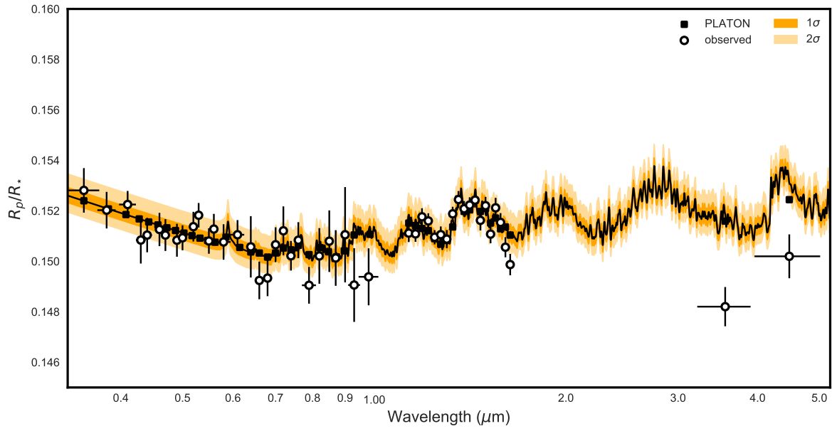
Figure 10. Transmission spectrum of HAT-P-32Ab measured with HST + Spitzer (open circles). The best-fit model binned to the resolution of the data (squares) and the median fit to the retrieved spectrum (black line) are shown. The shaded regions indicate the 1\sigma (medium orange) and 2\sigma (light orange) credible intervals.
