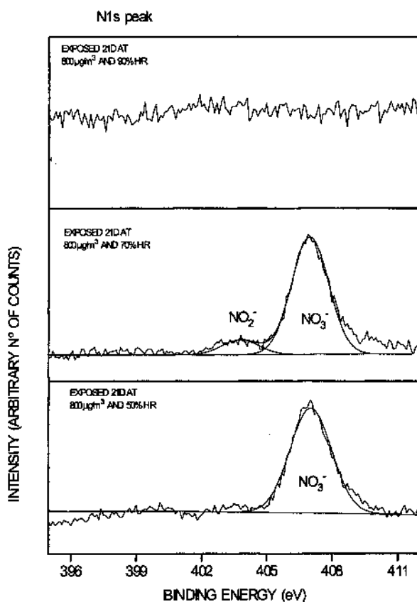
Figure 5. N1s high resolution XPS spectra obtained on the outer surface of copper specimens after 21 d of exposure in atmospheres contaminated with 800 \mu\text{g}/\text{m}^3 NO 2 at 50, 70 and 90 % RH.
