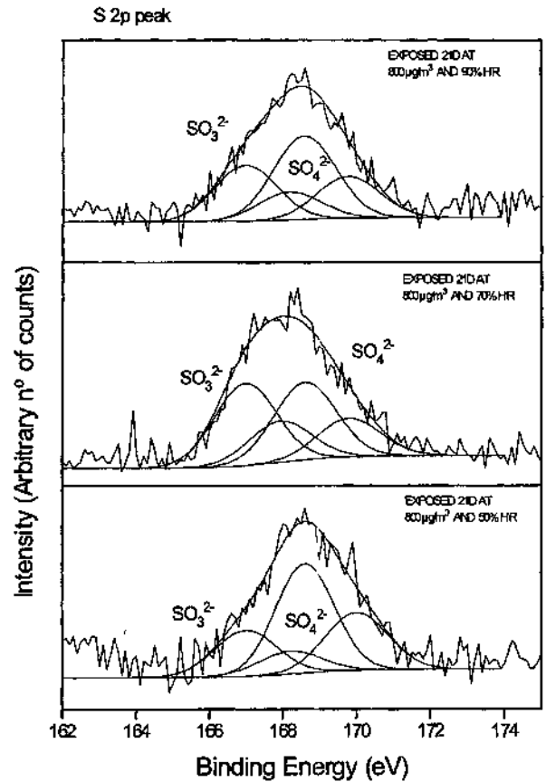
Figure 4. S2p high resolution XPS spectra obtained on the outer surface of copper specimens after 21 d of exposure in atmospheres with 800 \mu\text{g}\cdot\text{m}^{-3} \text{SO}_2 at 50, 70 and 90 % RH.
