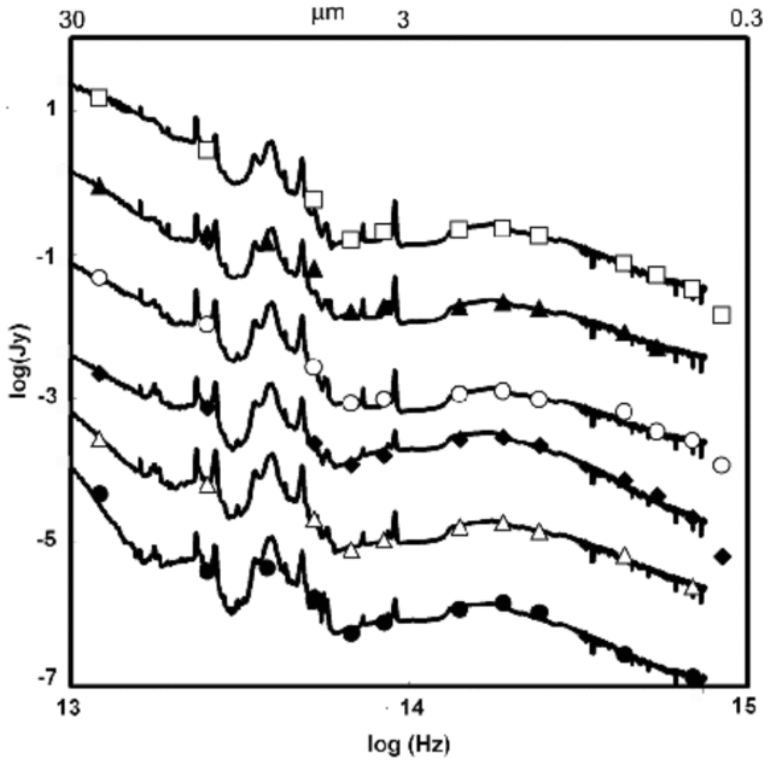
FIG. 2.— Expanded LIRG SEDs to highlight optical through mid-IR. The order of galaxies and offsetting factors are as in Figure 1.
