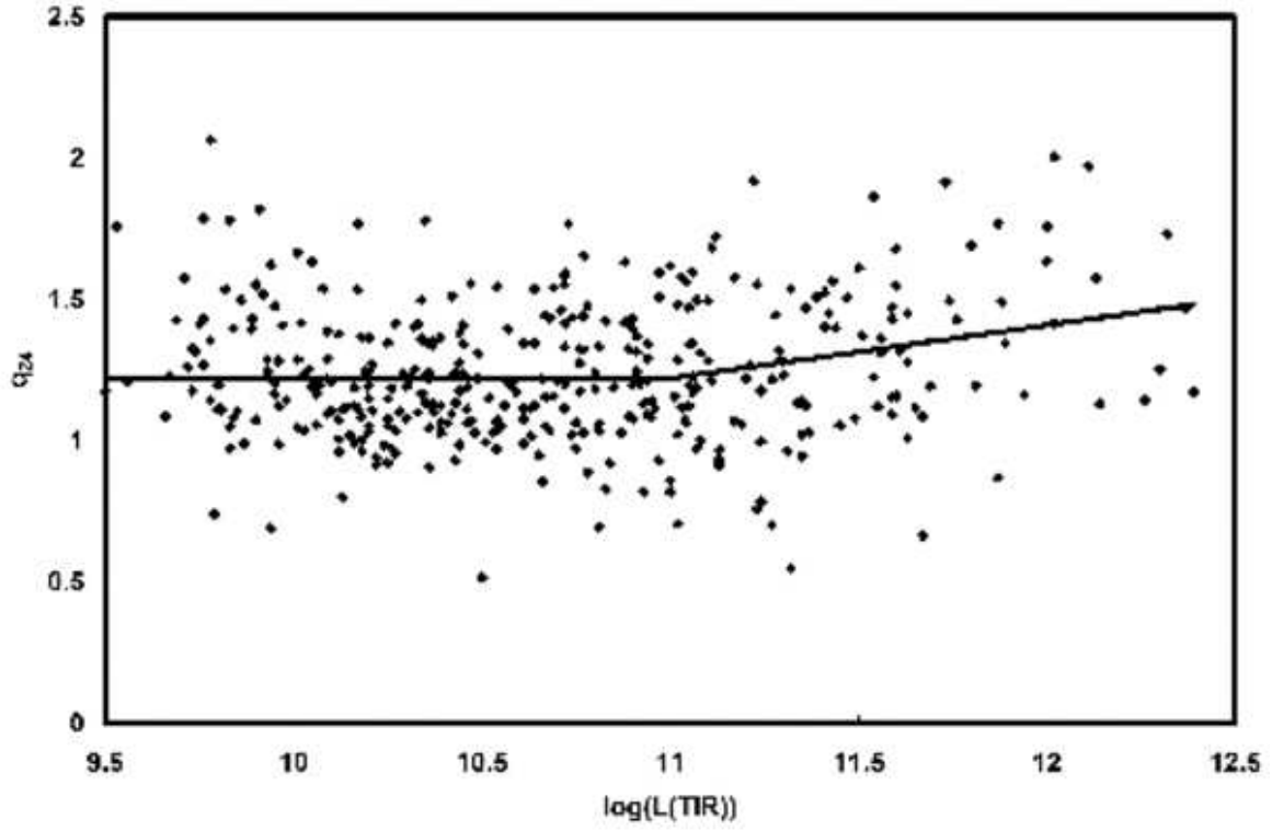
FIG. 11.— Trend of q_{24} = \log[f_{\nu}(24\mu\text{m})/f_{\nu}(1.4\text{GHz})] with \log(L(\text{TIR})) . The line shows our preferred fit, a constant of q_{24}=1.22 for \log(L(\text{TIR})) < 11 , and a sloping line above.
