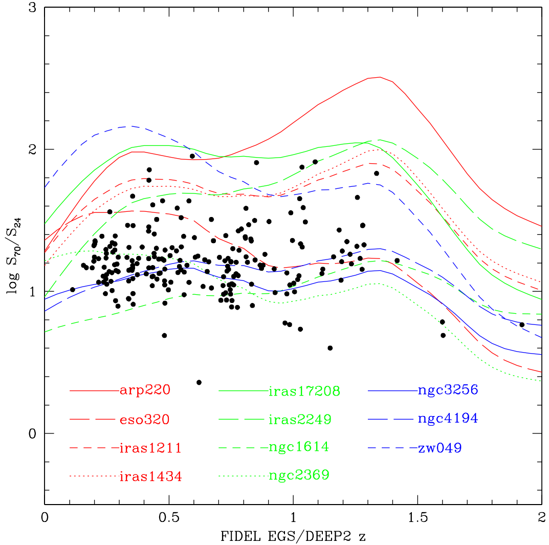
FIG. 17.— Behavior of templates in the far infrared. The templates have been redshifted and convolved with the MIPS relative response functions to predict their behavior at 24 and 70\mu\text{m} . The points show the ratios of 70 to 24\mu\text{m} flux densities in the EGS/FIDEL field for galaxies with L(TIR) > 5 \times 10^9 , and DEEP2 spectroscopic redshifts. Objects with low S_{70}/S_{24} are mostly AGN. For 0 < z < 1 , the templates define the space occupied by the measurements well. The "extra" template at low z is Zw 49.057, which evidently represents an anomalous spectral energy distribution not seen with any significant frequency in the FIDEL data. Above z \sim 1 , the sensitivity limitations at 70\mu\text{m} should result in a substantial bias in favor of sources with large 70/24 flux ratios and against those with small ratios. Nonetheless, compared with the locus of the family of templates, few such galaxies are identified. This result supports the work of Papovich et al. (2007) and Rigby et al. (2008) that indicate an increasing relative contribution of the \sim 8\mu\text{m} region to the total infrared outputs of galaxies at redshifts of z \sim 2 .
