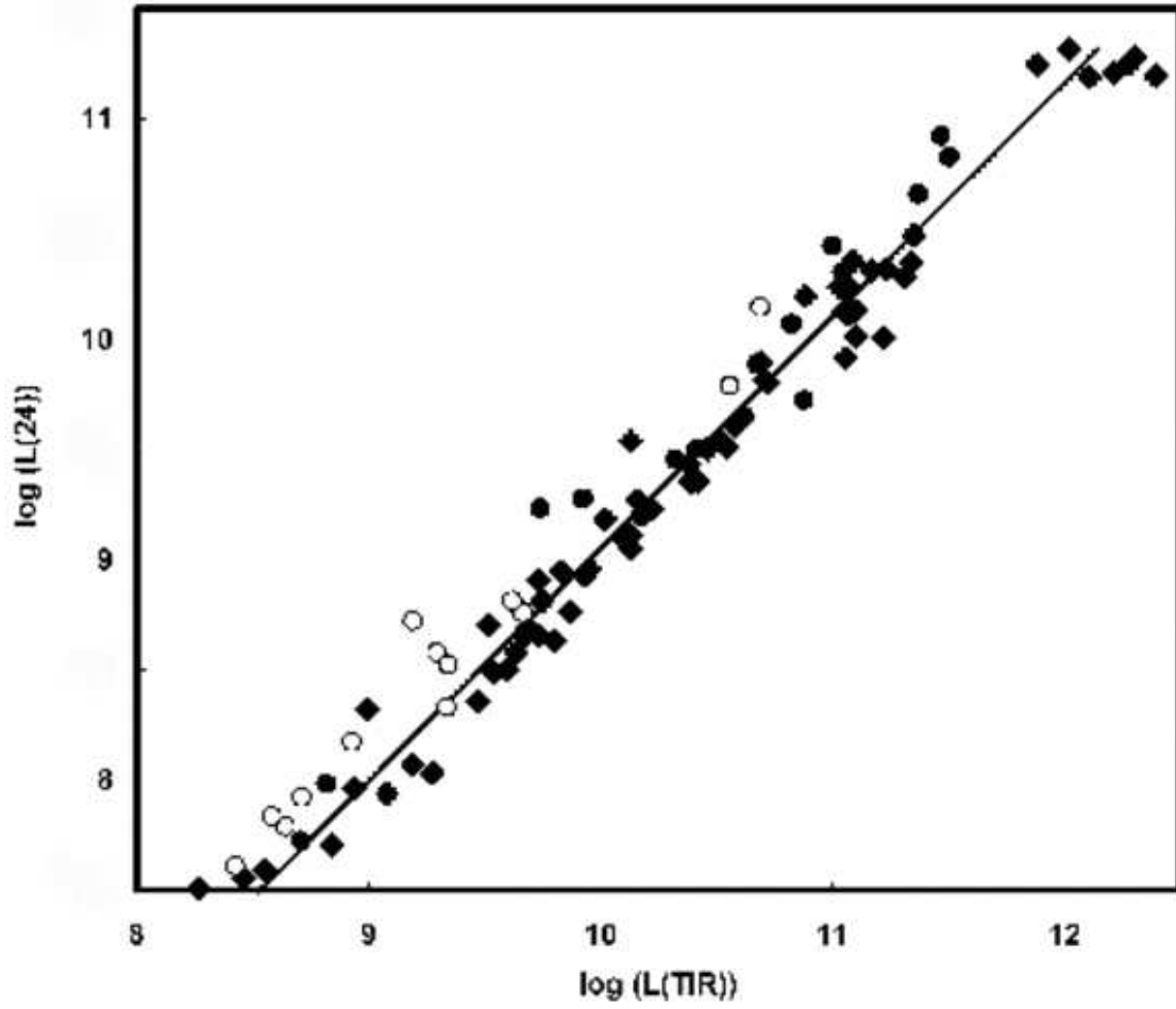
FIG. 15.— Comparison of L(24) and L(\text{TIR}) . The line is a linear fit as given in the text. It fits well with virtually no outliers and with a slope close to one (see Equation 25). Symbols are as for Figure 13.
