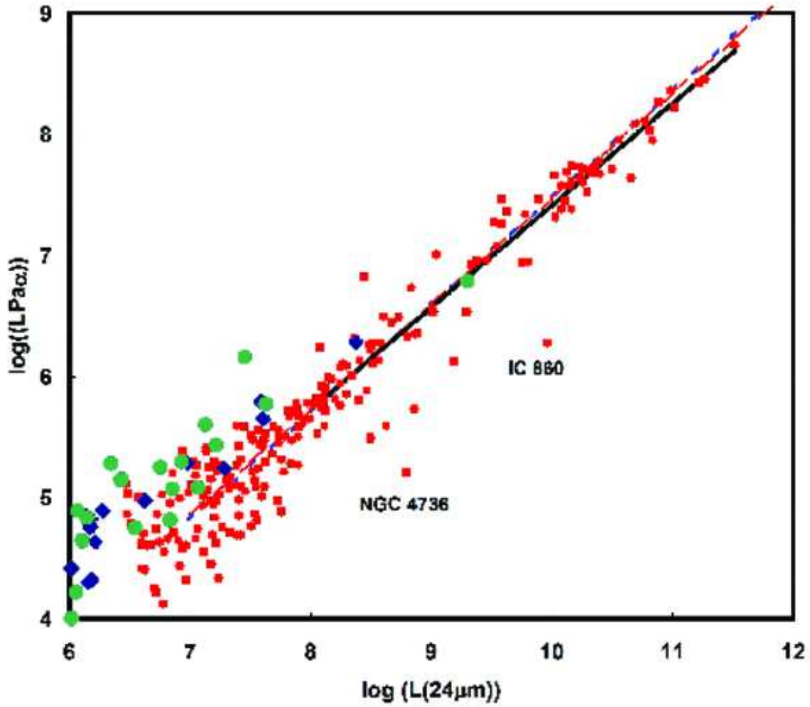
FIG. 7.— Comparison of Pa \alpha and 24 \mu\text{m} luminosities. The red squares are for high metallicity galaxies and HII regions as defined by Calzetti et al. (2007); the green circles are for intermediate metallicity; and the blue diamonds are for low metallicity. The fit (black line) is to the high metallicity points. The fits to subsets of the data by Alonso-Herrero et al. (2006) and Calzetti et al. (2007) are shown as dashed red and dashed blue lines, respectively.
