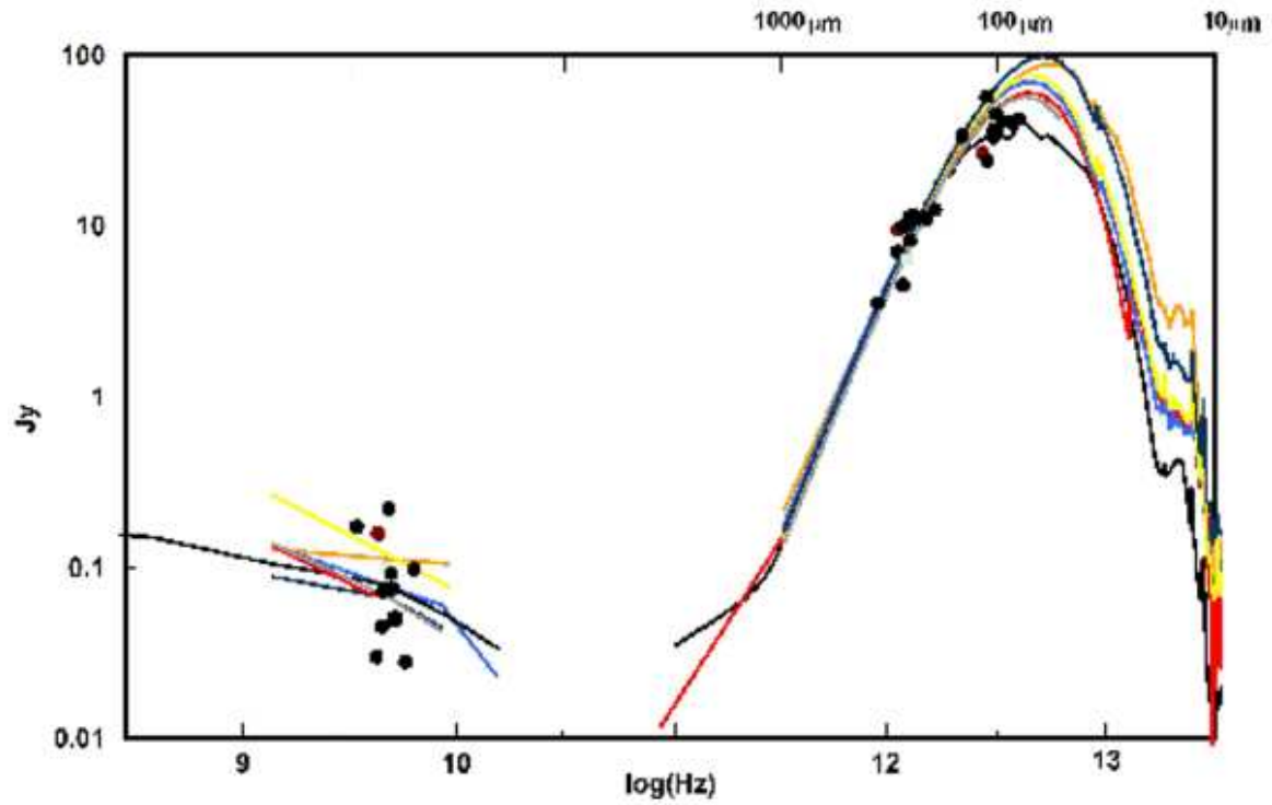
FIG. 12.— Comparison of our templates with the measurements of high redshift galaxies by Kovács et al. (2006). The templates and the measurements have all been normalized near 260\mu\text{m} , close to the rest wavelength for the 850\mu\text{m} measurements of Kovács et al. (2006). There is substantial scatter in the resulting radio fluxes for the templates but even more for the radio fluxes of the high redshift galaxies. The latter are perhaps increased significantly by measurement errors (not all of which are captured in the nominal errors, as demonstrated by the results of independent reductions (Kovács et al. 2006)). Nonetheless, the local templates are very representative of the behavior of those at high redshift.
