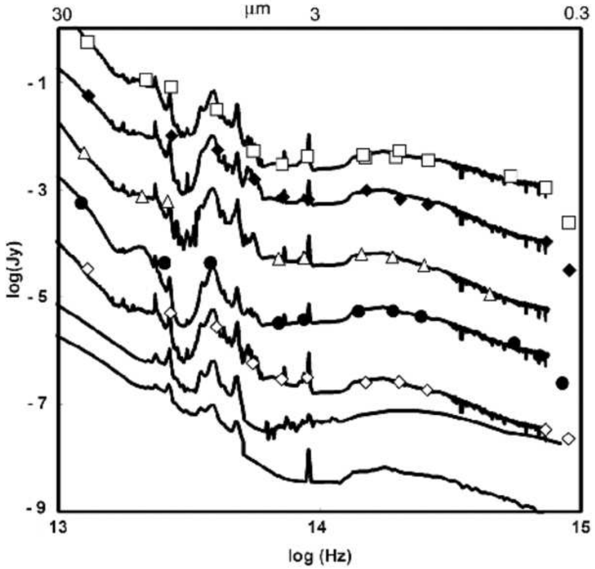
FIG. 4.— Expanded ULIRG SEDs to highlight optical through mid-IR. The order of galaxies and offsetting factors are as in Figure 3.
