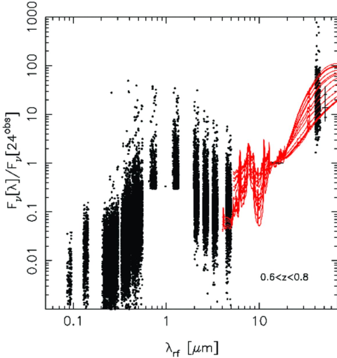
FIG. 18.— Comparison of templates with photometry at z \sim 0.7 . The photometry is for galaxies in the EGS with [3.6] < 23 (a cut that is responsible for the truncation of the distribution of points near 1 \mu\text{m} toward low values), photo- z between 0.6 and 0.8 (Perez-Gonzalez et al. 2008ab), a detection at 24 \mu\text{m} and/or 70 \mu\text{m} (as measured in the DR2 FIDEL data; Dickinson et al. 2007), and an estimated value of L(\text{TIR}) larger than 10^{11} L_{\odot} . The vertical line and marks on the right of the 70 \mu\text{m} fluxes show the median, quartiles and values enclosing 68% of the distribution of flux points. The templates and photometry are all normalized at observed 24 \mu\text{m} .
