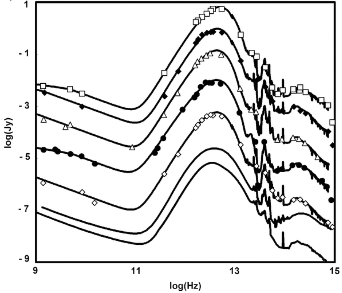
FIG. 3.— Full ULIRG SEDs and defining photometric points. Between 5 and 36\mu\text{m} the SEDs are based on IRS spectra rather than the photometry. The curves have been offset for clarity; from top to bottom the galaxies and offset factors are: 1.) IRAS 22491-1808 (1); 2.) IRAS 14348-1447 (0.1); 3.) IRAS 17208-0018 (0.003); 4.) Arp 220 (0.00007); 5.) IRAS 12112+0305 (0.00005); 6.) Dale \alpha = 1.5 model; and 7.) Chary & Elbaz L(\text{TIR}) = 2 \times 10^{12} model.
