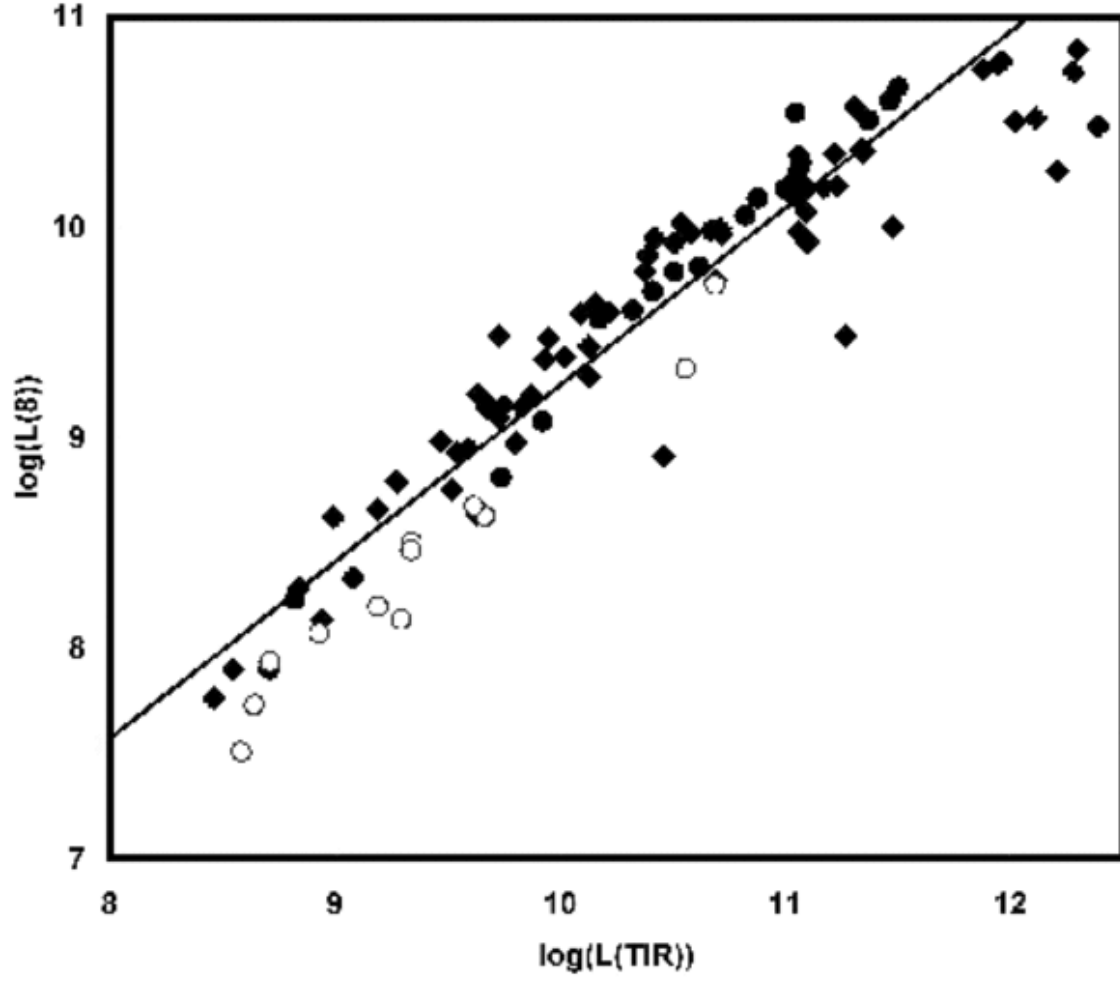
FIG. 13.— Comparison of L(8) and L(\text{TIR}) . Above \log(L(\text{TIR})) = 11 , the relation appears almost to saturate due to a number of very luminous galaxies with suppressed emission at 8\mu\text{m} . The diamonds are from Dale et al. (2007) and (for the LIRGs and ULIRGs) from our reduction of archival data. The circles are from Engelbracht et al. (2008); filled ones are within 0.25 dex of solar metallicity (in O/H) while open ones indicate metallicity between 0.25 and 0.5 dex below solar. The line is from Equation 21.
