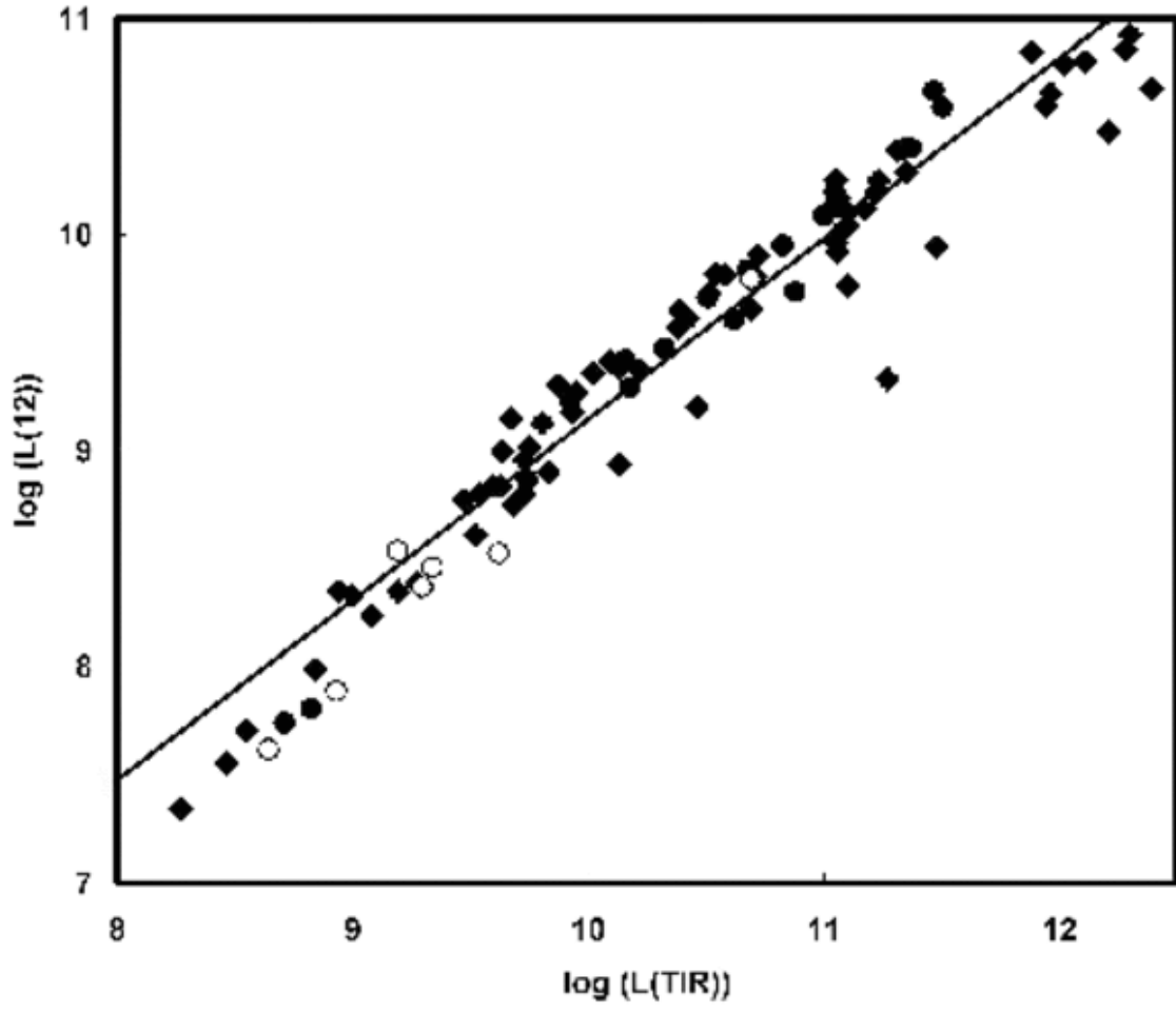
FIG. 14.— Comparison of L(12) and L(\text{TIR}) . The most deviant low point (NGC 1316) has been excluded from the fit. The slope is significantly different from one (see Equation 23) and there are indications of an overall curvature, with a lower ratio of L(12)/L(\text{TIR}) at high luminosity. Symbols are as for Figure 13.
