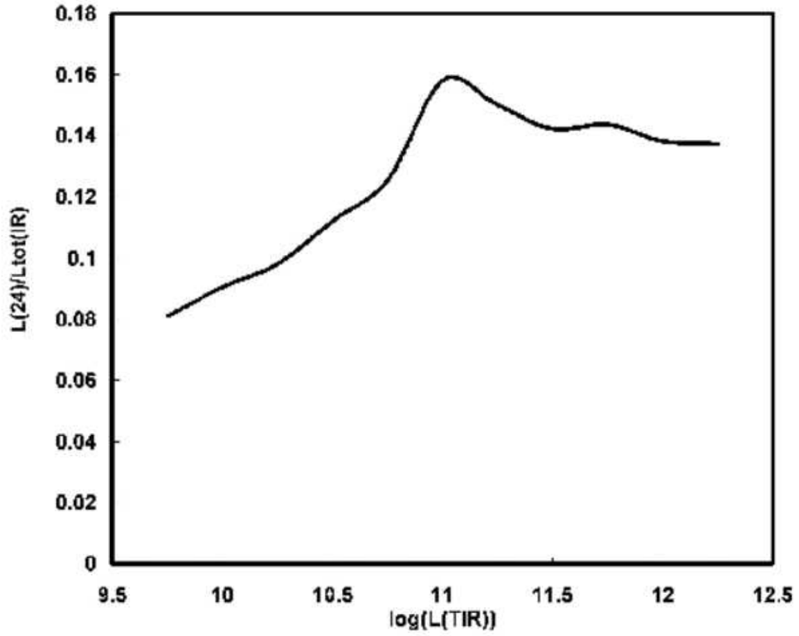
FIG. 8.— Trend of L(24)/L_{\text{tot}}(\text{IR}) with L(\text{TIR}) . L(\text{TIR}) is based strictly on the formulation of Sanders et al. (2003) using IRAS data, while L_{\text{tot}}(\text{IR}) is obtained by integrating under the infrared SED from 5 to 1000\mu\text{m} .
