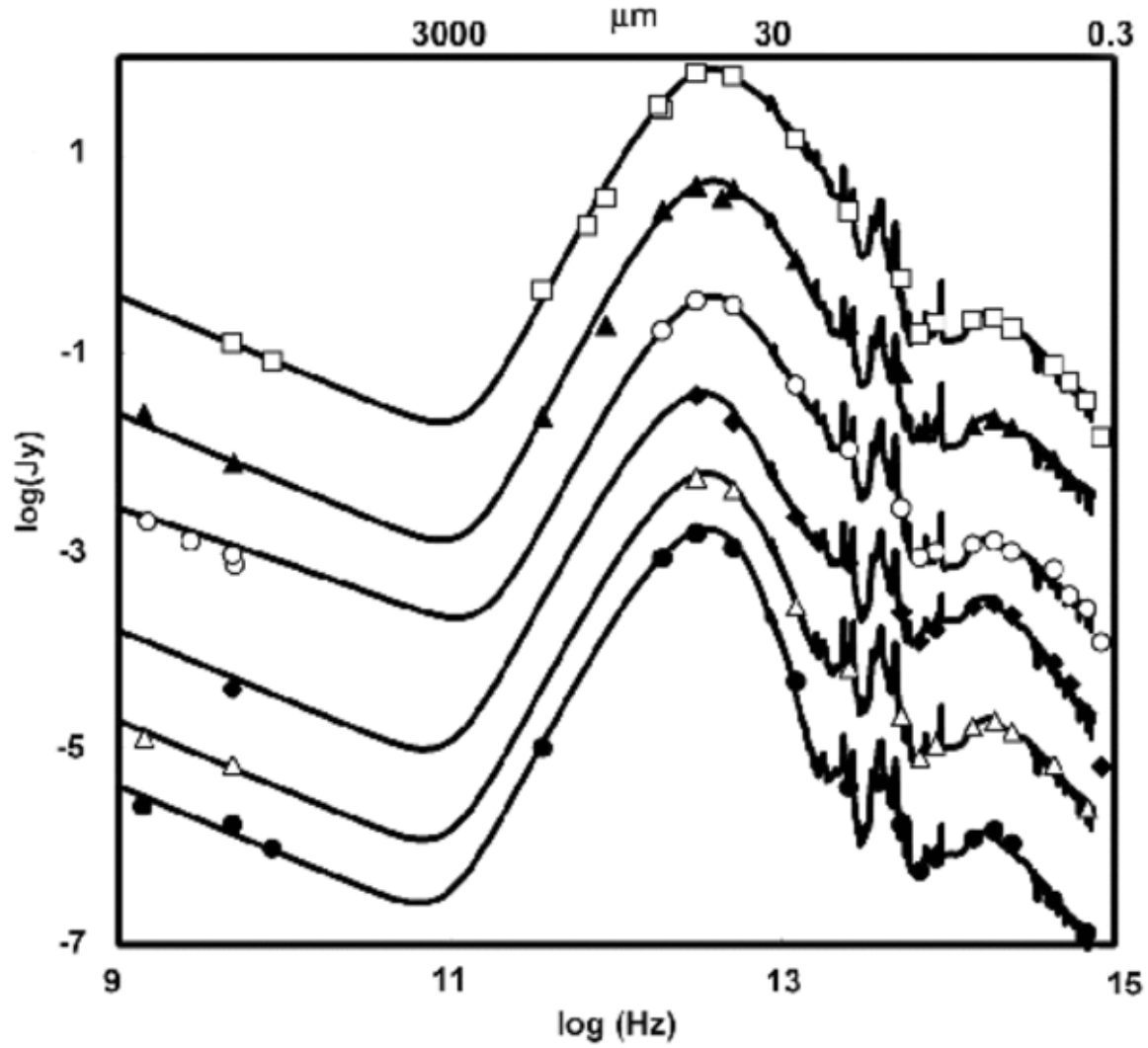
FIG. 1.— Full LIRG SEDs and defining photometric points. Between 5 and 36\mu\text{m} the SEDs are based on IRS spectra rather than the photometry. The curves have been offset for clarity; from top to bottom the galaxies and offset factors are: 1.) NGC 1614 (2); 2.) NGC 4194 (0.2); 3.) NGC 3256 (0.003); 4.) NGC 2369 (0.001); 5.) ESO 0320-g030 (0.0001); and 6.) Zw 049.057 (0.00005).
