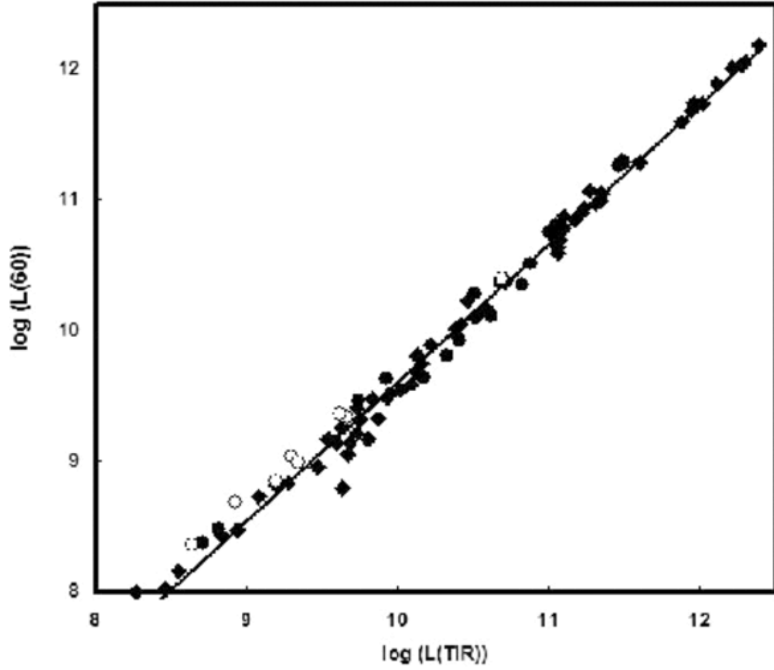
FIG. 16.— Comparison of L(60) and L(\text{TIR}) . The line is a linear fit given in the text. There are no outliers (not surprisingly because 60\mu\text{m} is close to the maximum of the SED) but the slope differs somewhat from unity (see Equation 26). Symbols are as for Figure 13.
