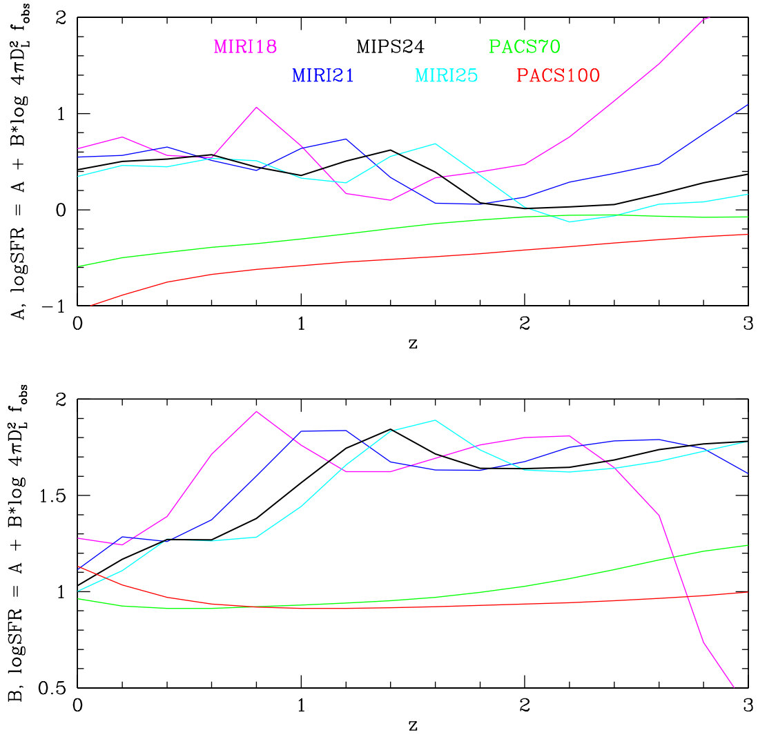
FIG. 10.— Trends with redshift of the intercept A and slope B for the relation between SFR and infrared flux, \log \text{SFR} = A + B(\log 4\pi D_L^2 f_\nu - 53) , for several infrared bands: Spitzer/MIPS 24\mu\text{m} (heavy black line); Herschel/PACS 70 and 100\mu\text{m} (green and red lines); JWST/MIRI 18 , 21 , and 25\mu\text{m} (magenta, blue, and cyan lines).
