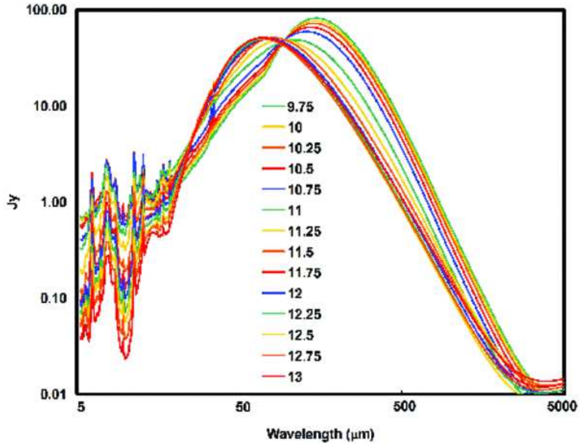
FIG. 6.— Family of average templates for full radio, far-infrared, and mid-infrared spectral range. The templates are keyed to the \log(L(\text{TIR})) of the galaxies, calculated as by Sanders et al. (2003). They are normalized to the same integrated flux. The templates for the three highest luminosities are extrapolated and are likely to be significantly less representative than the rest.
