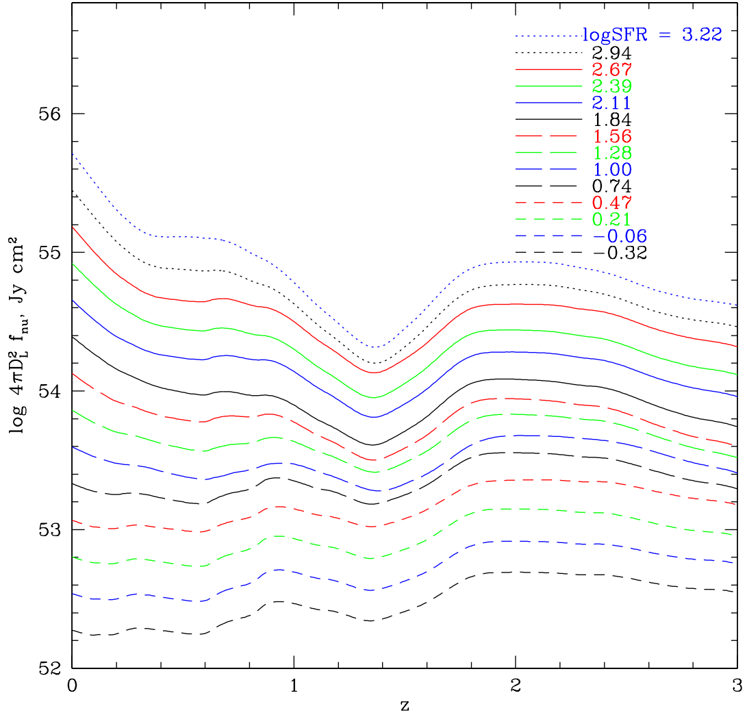
FIG. 9.— Tracks of the average template SEDs vs. redshift, as would be observed at 24\mu\text{m} . The even spacing at any given redshift implies that a power-law fit is a good approximation to the dependence of SFR on 24\mu\text{m} flux.
