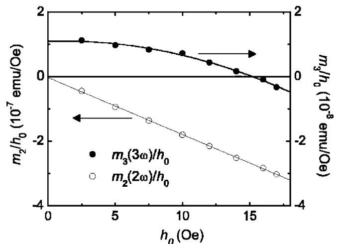
FIG. 1. Illustration of the method employed for measuring the nonlinear susceptibilities (here T=8 K, H_z=100 Oe, and \omega/2\pi=2 kHz). \chi_2(2\omega) and \chi_3(3\omega) are obtained, respectively, from the slope and the quadratic coefficient of the second m_2(2\omega)/h_0 and third m_3(3\omega)/h_0 harmonics of the output signal, measured as a function of the ac field amplitude h_0 .
