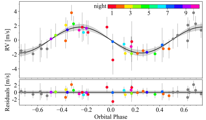
Figure 9. Phase folded RVs of the ten nights used to model the RV semi-amplitude of the USP planet using the FCO approach.
