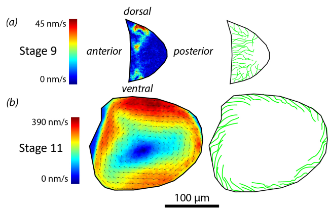
FIG. 1. Cytoplasmic streaming in the Drosophila oocyte. The 3D oocyte shape is approximately given by rotating the cross-section about its anterior-posterior axis. (a) Experimental flow field [28] and schematic of the disordered swirling flows and microtubule organization in early stages of development. (b) Later flows organize into a single vortex as MTs lie parallel to the cell periphery.
