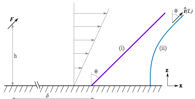
FIG. 5. Self-consistent model. An upstream point force \mathbf{F} parallel to the distal filament end produces shear flow that deflects the filament. Two variants: (i) rigid rod with a torsional spring at its base, (ii) a clamped elastic filament.
