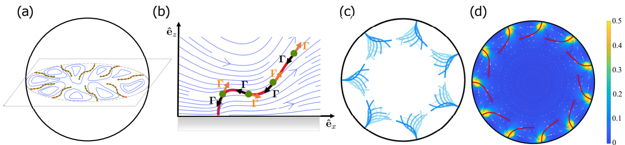
FIG. 2. Discrete filament computations. (a) N equally spaced filaments clamped at their attachment points, reach inward from a no-slip spherical shell. Each has a continuous distribution of tangential point forces (red) that (b) exert a force \mathbf{\Gamma} on the fluid and an equal and opposite compressive force on the filament. Synchronous oscillations ( N = 7 , \sigma = 1700 ), (d) steady, bent configuration ( N = 9 , \sigma = 500 ) and swirling flow field.
