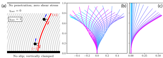
FIG. 3. Continuum model in planar geometry. (a) Bi-infinite array of MTs, clamped vertically at a no-slip boundary. Results of computations at (b) \rho = 4.65 , \sigma = 70 and (c) \sigma = 39 . Colors denote time, from cyan (early) to pink (late).
