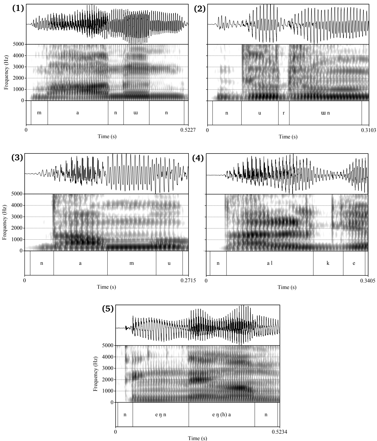
Figure 2. Examples of the five categories of realization of nasal phonemes in initial position: Category (1) Sonorant nasals [N]; Category (2) Partially denasalized nasals [N D ]; Category (3) (Pre-)voiced non-nasals [D]; Category (4) Voiceless non-nasals [T], and; Category (5) Voiceless non-nasals with a voicing lag of more than 10ms [T H ]. The tier below the spectrogram shows the underlying phonemes.
