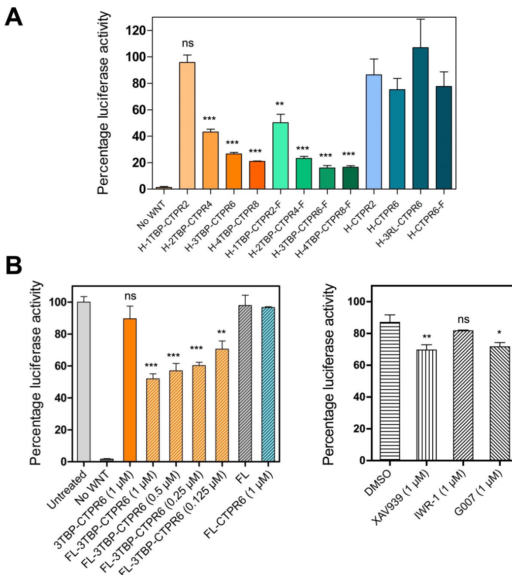
Figure 6. The effect on Wnt-activated HEK293T cells following treatment with the indicated HiBiT-tagged n TBP-CTPR _n constructs. (A) TOPFLASH reporter assay for HEK293T cells transfected with TCF-Firefly and Renilla reporter gene vectors and an expression vector encoding the constructs listed. For each sample, Luciferase activities were normalised with the Renilla values and the ratio was expressed as relative luciferase activity to the control well transfected with the empty HiBiT vector set at 100% (not shown in the graph). The monomeric constructs, trimeric constructs and controls are shown in different
