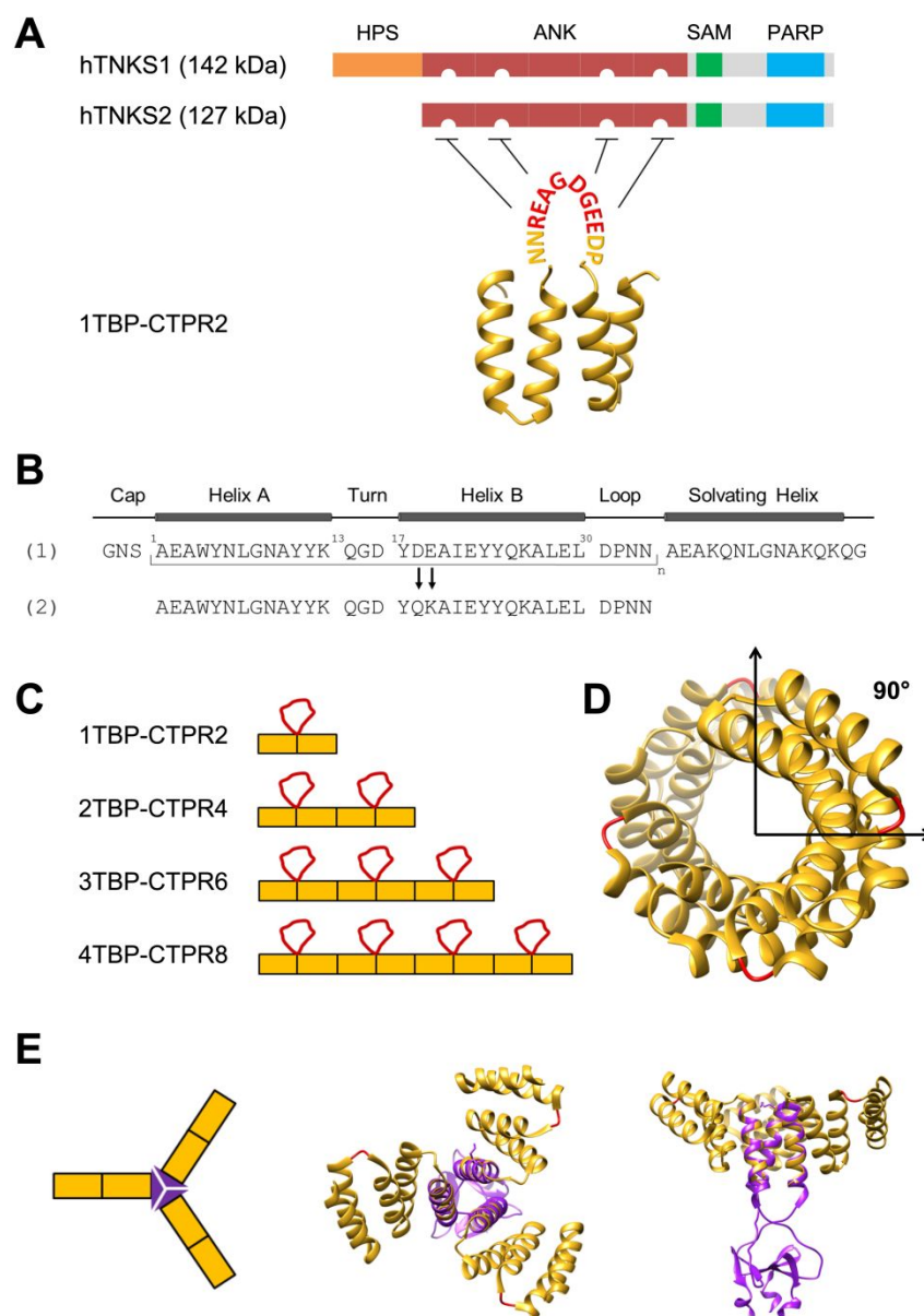
Figure 1. Design of hTNKS-binding CTPR proteins in different formats and valencies.
