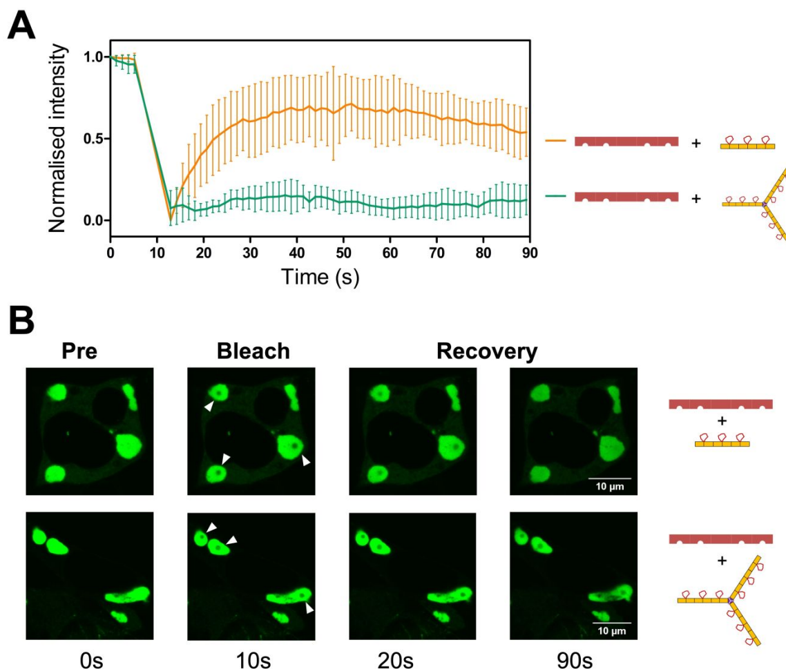
Figure 5. FRAP analysis of the assemblies formed between hTNKS2 ARC1-5 and TBP-CTPR proteins. (A) FRAP analysis was performed on seven individual Regions of Interest (ROI) selected within macromolecular assemblies induced by eGFP-tagged hTNKS2 ARC1-5 in complex with 3TBP-CTPR6 (orange) or 3TBP-CTPR6-foldon (green). HEK293T cells were bleached in the ROI and fluorescence recovery of eGFP-tagged hTNKS2 ARC1-5 was monitored over 90 seconds. (B) Representative ROI selected within three independent macromolecular assemblies are shown before, during and post bleaching.
