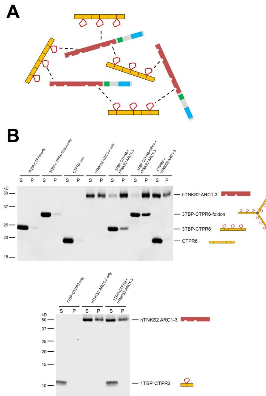
Figure 3: Multivalent interactions between TBP-CTPR proteins and hTNKS2 ARC1-3 analysed using a co-precipitation assay. (A) Schematic representation of the macromolecular assemblies formed by interaction of the multivalent hTNKS2 protein and the 3TBP-CTPR6 protein (used as representatives of the multivalent CTPR arrays). (B) After centrifugation, supernatant (S) and pellet (P) were separated and run on a 12% (top) or 16% (bottom) SDS polyacrylamide gel. For co-sedimentation, proteins were mixed in equal volumes at the following concentration: 10 \mu M 3TBP-CTPR6 (30 \mu M TBP loop concentration), 3.3 \mu M 3TBP-CTPR6-foldon (30 \mu M TBP loop concentration), 10 \mu M CTPR6 and 10 \mu M hTNKS2 ARC1-3 (20 \mu M TBP-binding sites). Gel images were obtained using Li-COR Odyssey Fc Imaging System.
