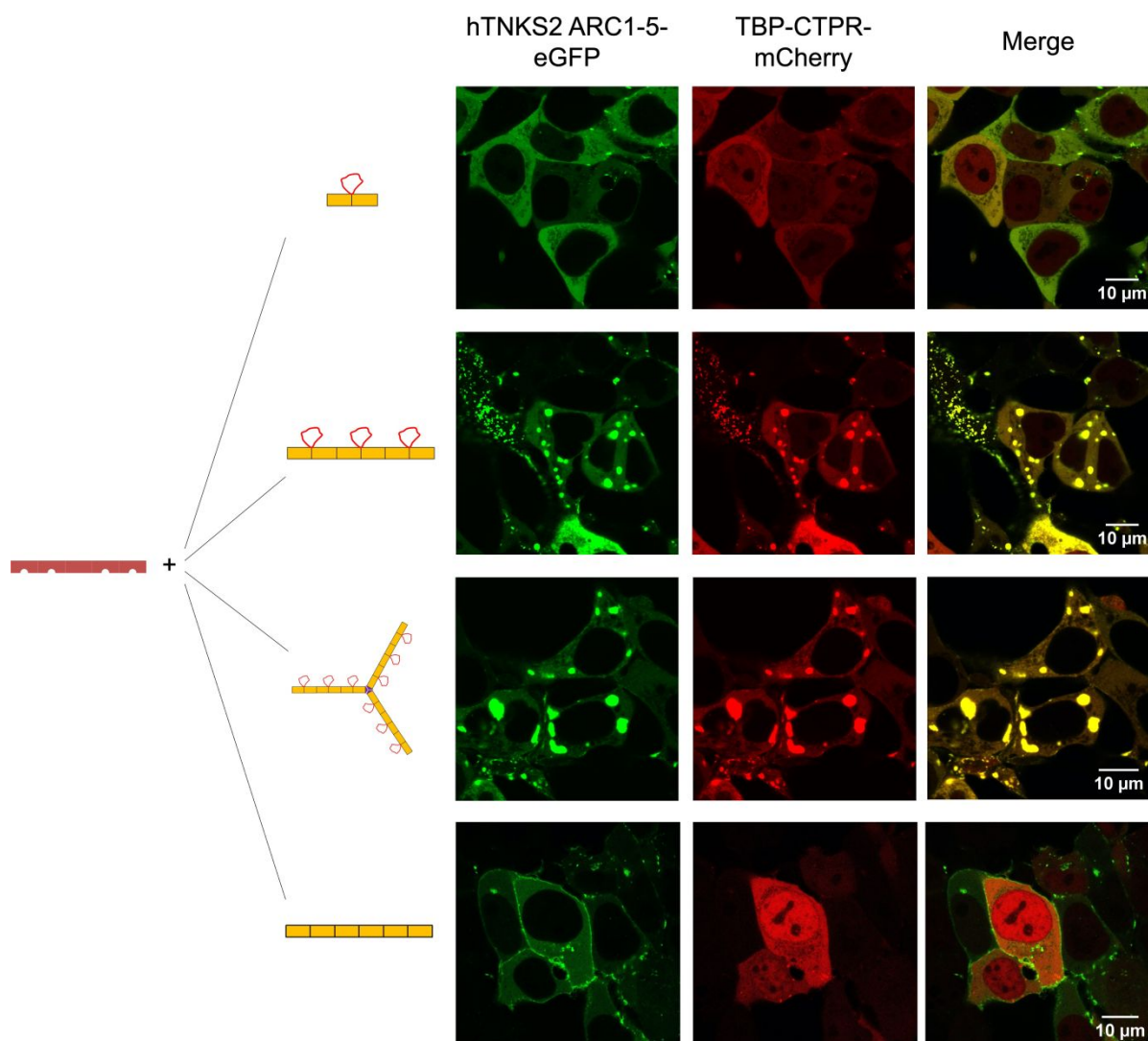
Figure 4. Fluorescence microscopy of HEK293T cells co-transfected with mCherry-tagged CTPR proteins and eGFP-tagged hTNKS2 ARC1-5. Co-localisation in large macromolecular clusters is observed for e-GFP-tagged hTNKS2 ARC1-5 in combination with mCherry-tagged 3TBP-CTPR6 or with mCherry-tagged 3TBP-CTPR6-foldon. These clusters are not observed for the mono-valent mCherry-tagged 1TBP-CTPR2 protein or the control mCherry-tagged CTPR6 protein. Scale bars for all images are 10 µm.
