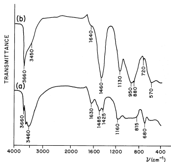
Figure 5. FTIR Analyses of the MSWIFA: a) before and b) after 1 hour of HT.
