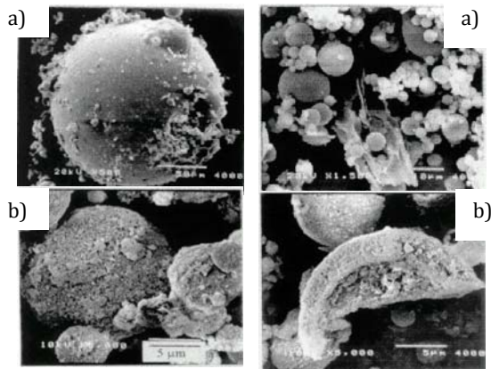
Figure 2. Morphologic of fly ash before (a) and alter hidrothermal treatment (b)
