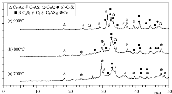
Figure 3. XRD diffractograms of FABC with calcinations temperature
