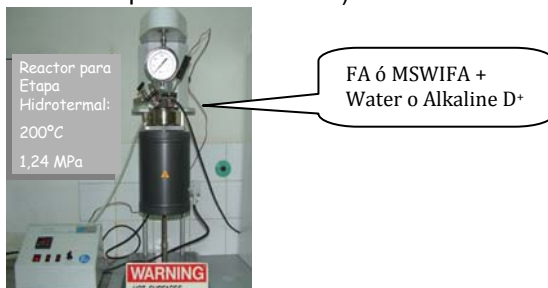
Figure 1. Hydrothermal Step: Cement Precursors Phases
