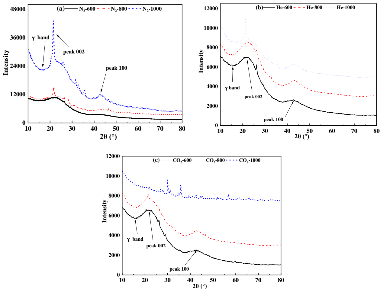
Fig.5. The X-ray diffraction patterns of biochar prepared at 600, 800 and 1000 °C under (a) N 2 atmosphere, (b) He atmosphere and (c) CO 2 atmosphere.
