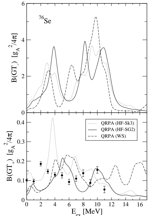
FIG. 7. Same as in Fig. 6, but for ^{76}\text{Se} . Data are from Ref. [29].
