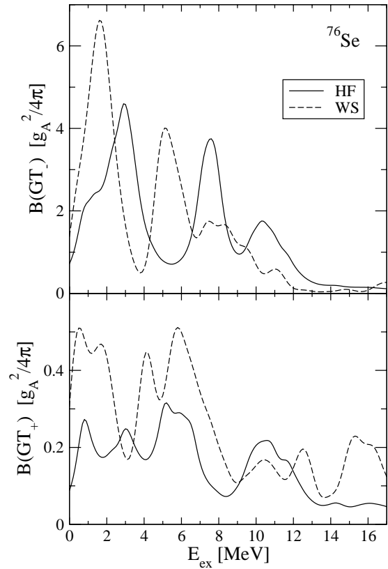
FIG. 3. Same as in Fig. 2, but for ^{76}\text{Se} .
