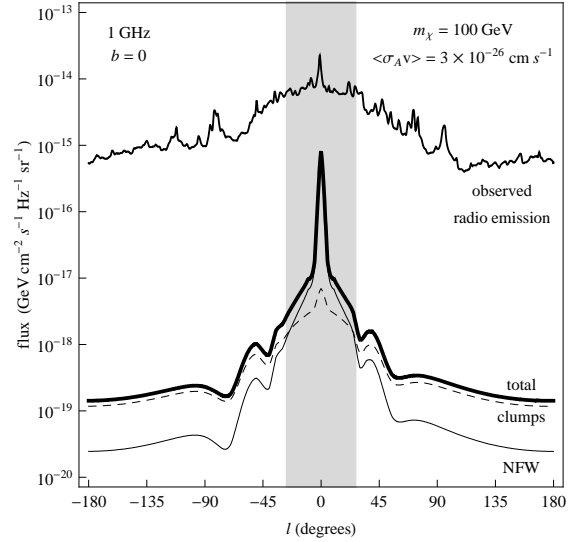
FIG. 5: DM synchrotron profile for the halo and unresolved substructures and their sum at 1 GHz for m_\chi = 100 GeV and \langle\sigma_A v\rangle = 3 \times 10^{-26} \text{cm}^3 \text{s}^{-1} . The astrophysical observed emission at the same frequency is also shown. The gray band indicates the angular region within which the DM signal from the host halo dominates over the signal from substructures modeled as in section II A.
