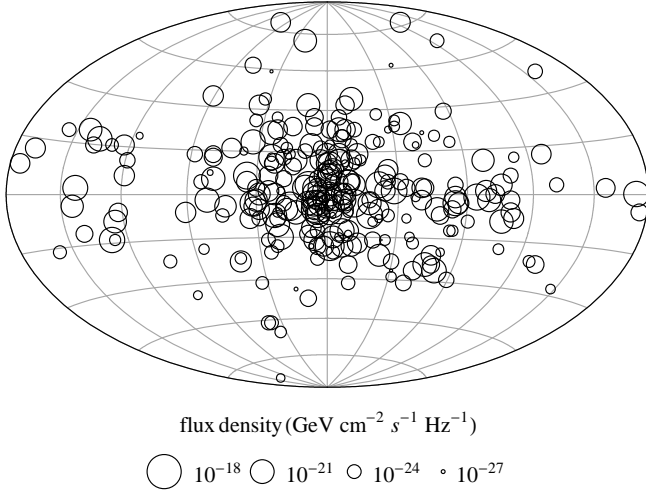
FIG. 4: Sky map at the frequency of 1 GHz for a realization of clumps distribution. For each clump, the circle radius is proportional to the logarithm of radio flux.
