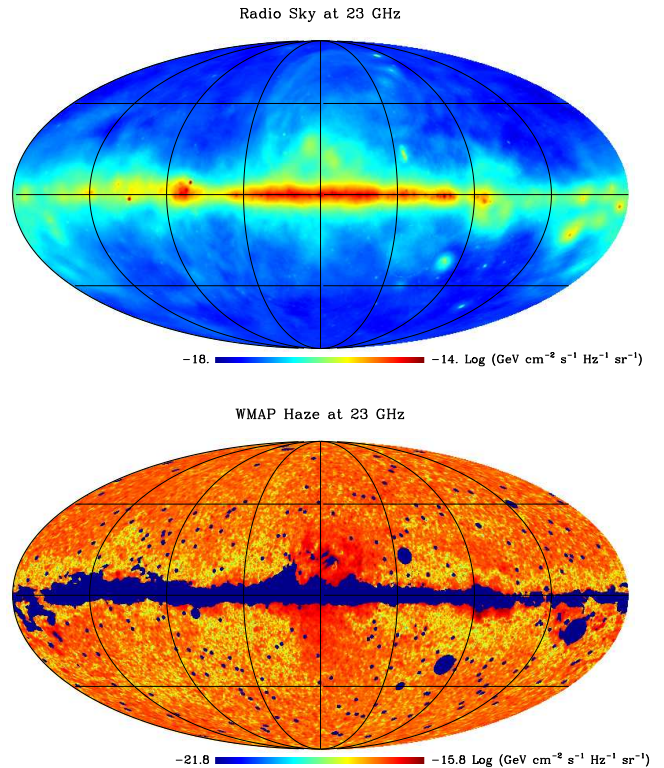
FIG. 1: Sky map of galactic foregrounds at the frequency of 23 GHz (top), and of the residual map showing the WMAP Haze (bottom).
