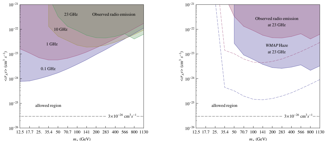
FIG. 7: (Left) Constraints in the m_\chi - \langle\sigma_A v\rangle plane for various frequencies without assuming synchrotron foreground removal. (Right) Constraints from the WMAP 23 GHz foreground map and 23 GHz foreground-cleaned residual map (the WMAP Haze) for the TT model of magnetic field (filled regions) and for a uniform 10 \mu\text{G} field (dashed lines).
