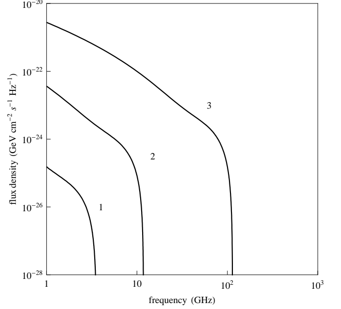
FIG. 3: Synchrotron flux density from three different clumps. The neutralino parameters are m_\chi c^2 = 100 \text{ GeV} and \langle \sigma_A v \rangle = 3 \times 10^{-26} \text{ cm}^3 \text{s}^{-1} , while the relevant clumps parameters are shown in table II.
