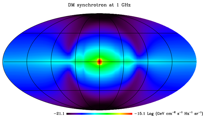
FIG. 6: Sky map of the galactic radio signal generated by the DM smooth halo and unresolved clumps at the frequency of 1 GHz for m_\chi = 100 GeV and \langle\sigma_A v\rangle = 3 \times 10^{-26} \text{cm}^3 \text{s}^{-1} . The peculiar shape of the signal, pinched approximately at \pm 30^\circ and \pm 60^\circ , reflects basically the structure of the magnetic field as seen in projection from the Solar System, where the observer is located (compare also with Fig.2). The galactic center region and the first few magnetic arms are visible as regions of high magnetic field intensity and hence prominent synchrotron emission.
