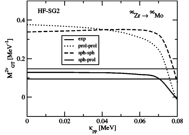
FIG. 19. 2\nu\beta\beta -decay matrix elements of ^{96}\text{Zr} obtained from Skyrme (SG2) deformed Hartree-Fock calculations as a function of the particle-particle interaction strength \kappa_{GT}^{pp} . The dotted curve corresponds to calculations using the prolate shapes for parent and daughter \beta_p=0.147 , \beta_d=0.119 (see Table II). The dashed curve is for spherical shapes and the solid curve is for spherical parent and prolate daughter \beta_p=0.016 , \beta_d=0.119 (see Table II). Horizontal lines are the experimental M_{GT}^{2\nu} extracted from Ref. [34] using g_A=1.0 and g_A=1.25 .
