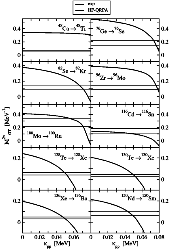
FIG. 18. 2\nu\beta\beta -decay matrix elements obtained from Skyrme (Sk3) deformed Hartree-Fock calculations as a function of the particle-particle interaction strength \kappa_{GT}^{pp} . Horizontal lines are the experimental M_{GT}^{2\nu} extracted from Ref. [34] using g_A=1.0 and g_A=1.25 .
