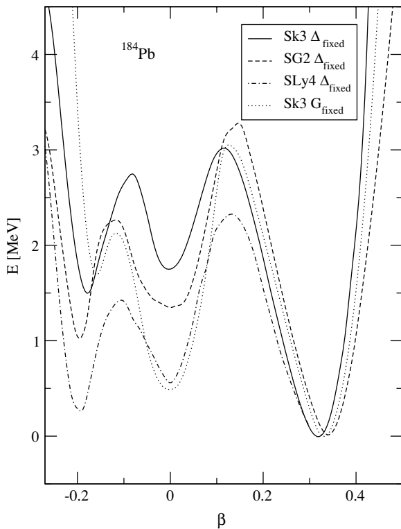
FIG. 2. HF energy of ^{184}\text{Pb} as a function of the quadrupole deformation \beta for various forces and pairing treatments.
