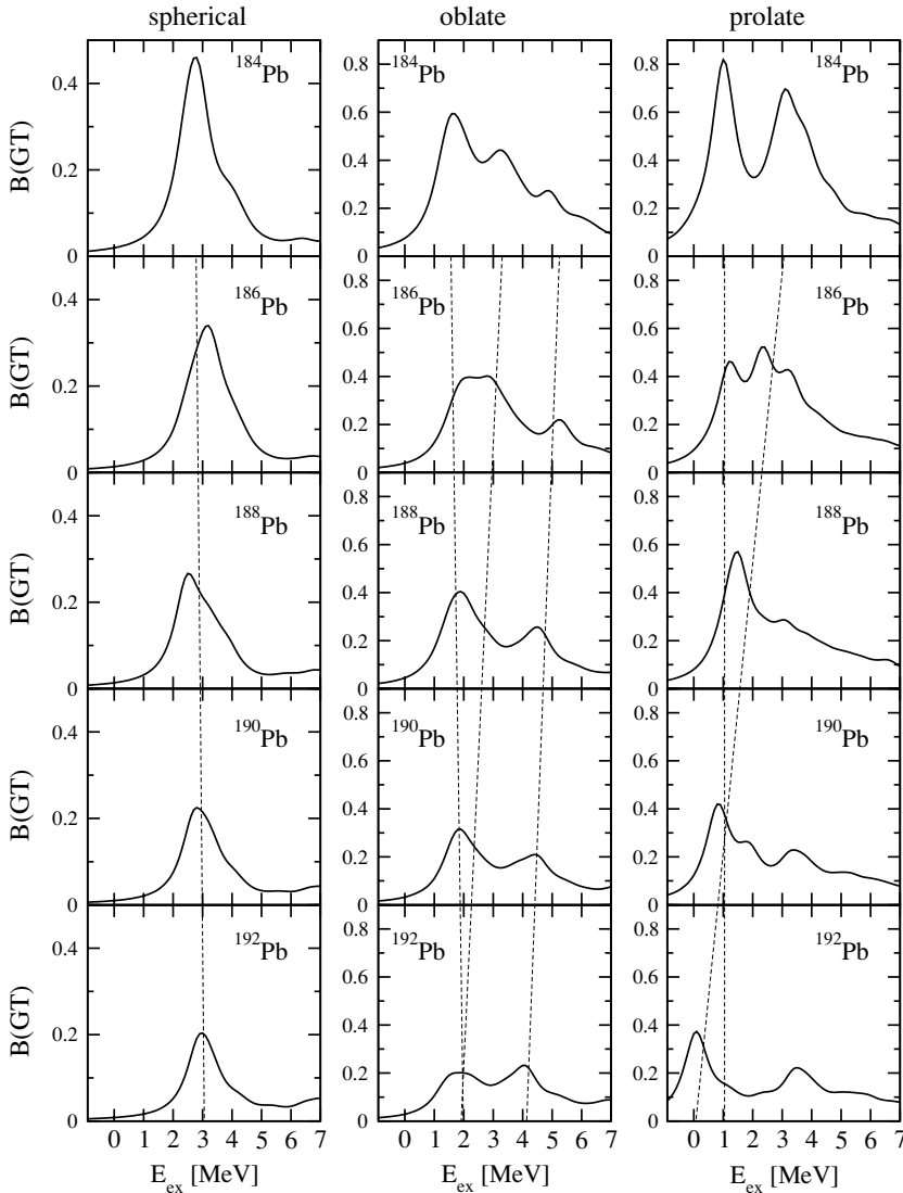
FIG. 5. Gamow-Teller strength distributions in the ^{184,186,188,190,192}\text{Pb} isotopes for spherical (left), oblate (middle), and prolate (right) shapes. Results are obtained from Sk3 force with fixed gap parameters.
