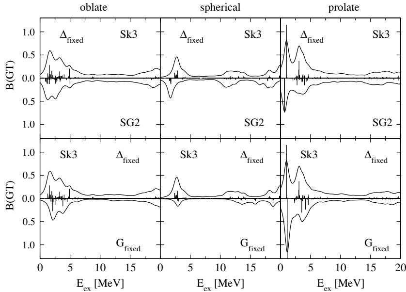
FIG. 4. Gamow-Teller strength distributions in ^{184}\text{Pb} as a function of the excitation energy in the daughter nucleus. From left to right we show the results for oblate, spherical, and prolate shapes. In the upper panels we show the results from Sk3 (upward) and SG2 (downward) with fixed gap parameters, whereas in the lower panels we show the results from fixed pairing gaps (upward) and constant pairing strengths (downward) for Sk3.
