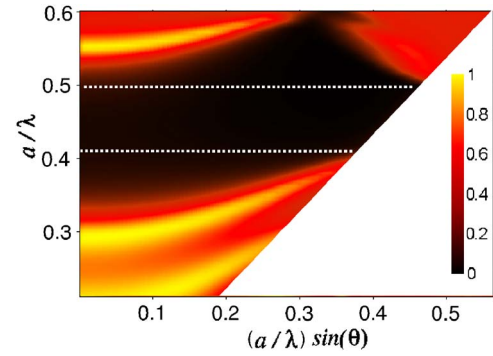
FIG. 2. (Color online) Ratio of transmitted to the incident power for a finite slab of a square lattice ( 4 \times 60 ) of Si rods in a map of frequency ( a/\lambda ) vs transversal momentum of the incoming radiation (a/\lambda) \sin \theta_0 .
