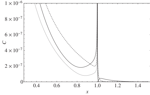
FIG. 1. Concurrence of the atomic state in the electromagnetic vacuum \rho_{AB}^{(0)} as a function of x=L/ct for three values of z = \Omega L/c = 5 (solid line), 10 (dashed line), and 15 (dotted line). The height of the peak is C^{(0)}=1 .
