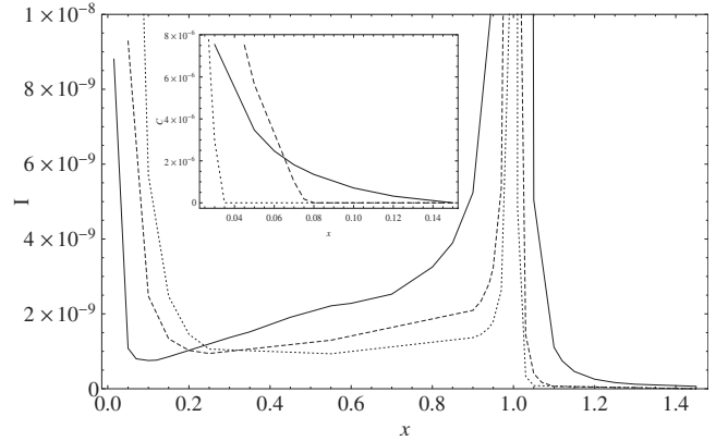
FIG. 3. Mutual information of \rho_{AB} as a function of x=L/ct for z=\Omega L/c=5 (solid line), 10 (dashed line), and 15 (dotted line). The inset shows the finite concurrences that are possible only for small values of x .
