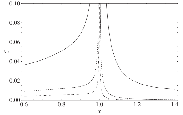
FIG. 2. Concurrence for one photon final state (10) as a function of x=L/ct for three values of z=\Omega L/c=5 (solid line), 10 (dashed line), and 15 (dotted line). Entanglement vanishes as t \rightarrow \infty ( x \rightarrow 0 for a given L ) and is sizable for x > 1 .
