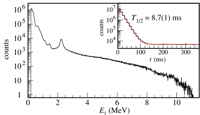
FIG. 1 (color online). Energy spectrum of ( E_1, t_1 ) events, defined as those following a ^{11}\text{Li} implantation in the same pixel within 40 ms: These are ^{11}\text{Li} decays. The inset shows the time behavior of all events following an implantation: The short-time component has the expected ^{11}\text{Li} half-life.
