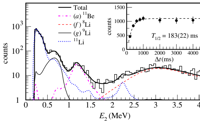
FIG. 2 (color online). Example of a fit of (E_2, t_2) events, with contributions from daughter decays in channels (a), (f), and (g), and uncorrelated ^{11}\text{Li} decays. This spectrum was obtained for t_2 - t_1 < 200 ms and for E_1 between 0.5 and 2.0 MeV. The inset shows the number of ^9\text{Li} decay events in the (E_2, t_2) spectra for t_2 - t_1 < \Delta t as function of \Delta t . The fitted time behavior is in agreement with the expected ^9\text{Li} half-life T_{1/2} = 178.3(4) ms [19].
