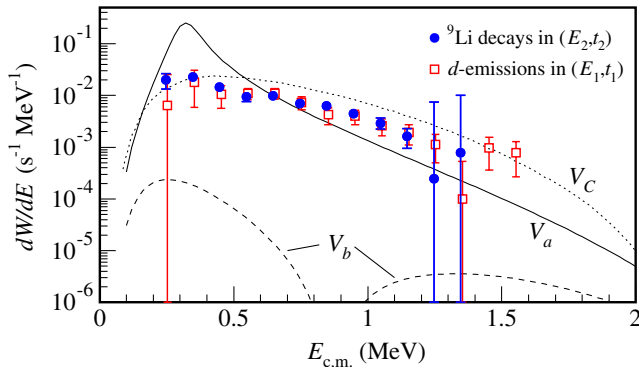
FIG. 3 (color online). Transition probability for the ^{11}\text{Li} \rightarrow ^9\text{Li} + d decay channel. The procedures to obtain the experimental data are explained in the text. The curves are predictions from Refs. [7] ( V_C ) and [8] ( V_a and V_b ).
