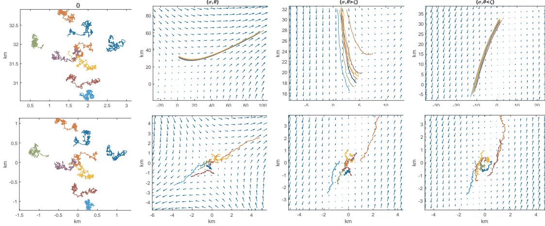
Figure 1: Simulation of 9 drifters from equation (2) over 6.25 days, with starting positions, number of drifters, and length of experiment taken to match LatMix Site 1. In each panel the submesoscale velocities \{u_k^{\text{sm}}(t), v_k^{\text{sm}}(t)\} follow a Wiener increment process with diffusivity equal to 0.1 \text{ m}^2/\text{s} . The top row shows drifter positions, and the bottom row shows positions with respect to centre-of-mass at each time step. From left to right we include the following model components. Left: diffusivity only. Centre left: strain and diffusivity. Centre right: strain, vorticity, and diffusivity (strain dominated). Right: strain, vorticity, and diffusivity (vorticity dominated). In each plot where a parameter is present, it has been set as \kappa = 0.1 \text{ m}^2/\text{s} , \sigma = 7 \times 10^{-6}/\text{s} , \theta = 30^\circ , \zeta = 6 \times 10^{-6}/\text{s} (centre right), and \zeta = 8 \times 10^{-6}/\text{s} (right). We have set u_0 = v_0 = u_1 = v_1 = u^{\text{bg}} = v^{\text{bg}} = 0 . The trajectories are simulated using the Euler-Maruyama scheme.
