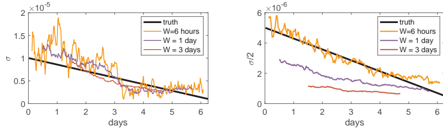
Figure 7: The left panel shows rolling-time window estimates of the varying strain rate from the data presented in Figure 6 over 3 choices of window lengths using the second-moment fitting method. The right panel shows the standard error of these time-varying estimates over 100 repeated simulations, plotted against \sigma/2 .
