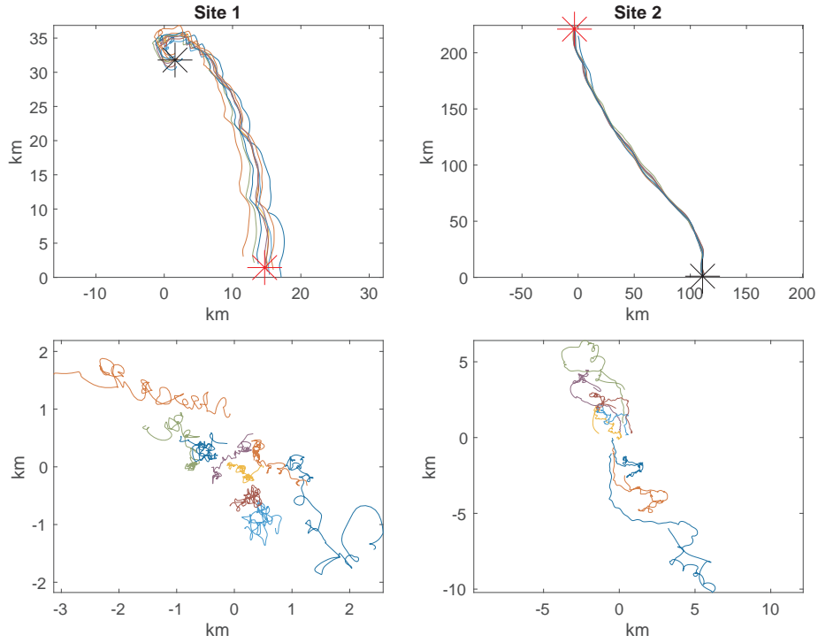
Figure 10: LatMix trajectories of Site 1 (9 drifters) and Site 2 (8 drifters). Top row are the positions in \{x_k(t), y_k(t)\} , bottom row relative to centre-of-mass \{\bar{x}_k(t), \bar{y}_k(t)\} = \{x_k(t) - \frac{1}{K} \sum_{k=1}^K x_k(t), y_k(t) - \frac{1}{K} \sum_{k=1}^K y_k(t)\} . The black and red star in the top row of plots indicate the respective starting and ending centre-of-mass positions. \{0, 0\} in the \{x, y\} components corresponds to \{-73.0234, 31.7424\} degrees longitude-latitude for Site 1 and \{-73.6776, 32.2349\} degrees longitude-latitude for Site 2.
