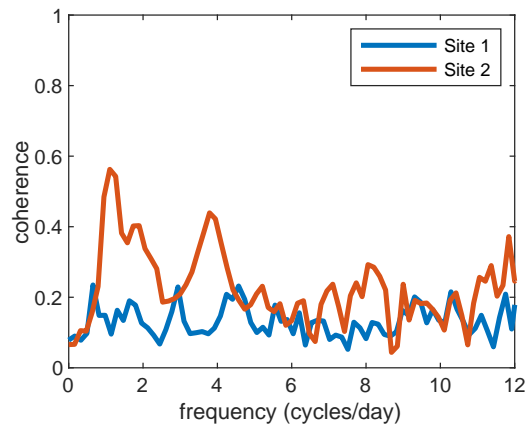
Figure 16: Coherence between the mesoscale signal in the centre-of-mass frame and the sub-mesoscale signal at Site 1 and Site 2, using the disentangled velocities corresponding to the trajectories shown in Figures 14 and 15 respectively.
