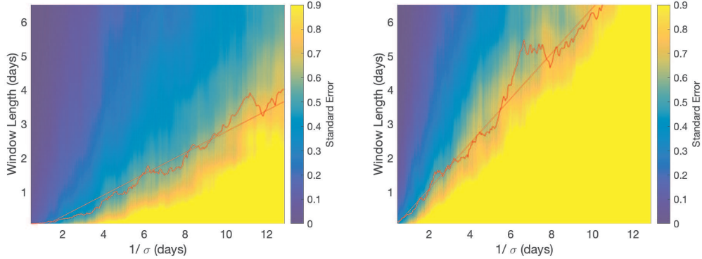
Figure 8: Estimated standard errors for the strain rate (in the units of the true strain rate) across a dense grid of fixed strain rate values \sigma and window lengths W in a strain-only simulation mirroring the setup in Figure 1. In the left panel we have set \kappa = 0.1 \text{ m}^2/\text{s} and in the right \kappa = 1 \text{ m}^2/\text{s} . The strain rate estimates are obtained using the second-moment fitting method of a strain-only model, and the standard errors are obtained using the jackknife (a variant of the bootstrap which is computationally faster to implement and was found to perform similarly). The standard errors in the heatmap are upper-bounded by 0.9 for representation purposes. We draw a red line (and best fit regression line) where the standard error is half the true parameter value for each value of the strain rate.
