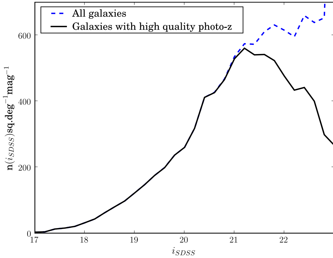
Fig. 9.— Differential number counts distribution of L > L_* red galaxies.
