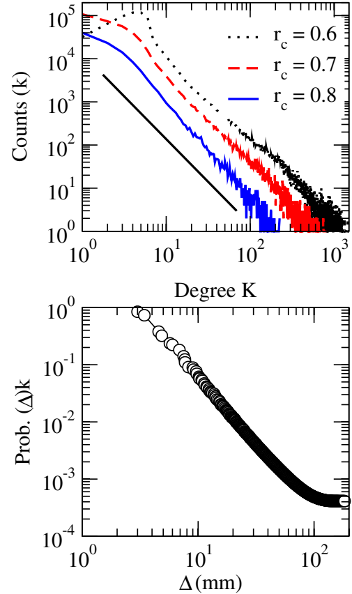
FIG. 3 (color online). Average scaling taken from 22 networks extracted from seven subjects. Top Panel: Average degree distribution. The straight line illustrates a decay of k^{-2} . Bottom panel: Average probability of finding a link between two nodes separated by a distance larger than \Delta (using r_c = 0.6 ).
