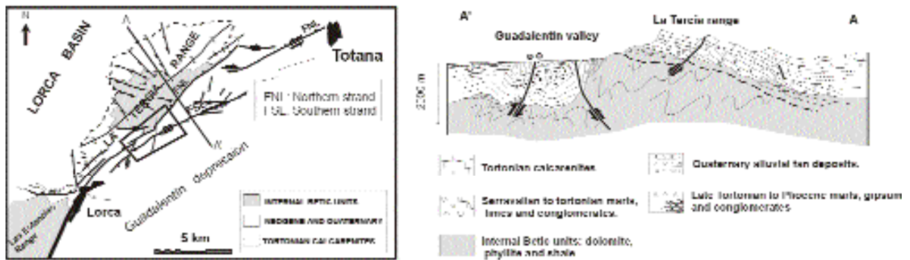
Figure 2. Geological cross section transversal to the Alhama de Murcia fault zone (Lorca-Totana sector) showing the two strands of this fault and the structure of the La Tercia range linked to the reverse slip of the northern fault. See location in the map.
