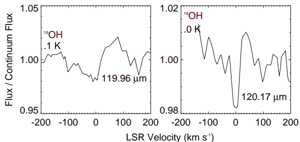
Figure 14. ^{18}\text{OH} lines observed in the survey towards Orion KL. The left plot is the ^2\Pi_{3/2} 5/2^+ \rightarrow 3/2^- transition at 119.96 \mu\text{m} and the right plot is the ^2\Pi_{3/2} 5/2^- \rightarrow 3/2^+ transition at 120.17 \mu\text{m} .
