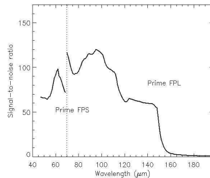
Figure 4. The signal to noise achieved for the L03 prime-detector spectra. Peaks in the curve represent the spectral ranges with the highest data reliability. The vertical dotted line divides the spectral ranges observed by the short wavelength FP (FPS) from those observed by the long wavelength FP (FPL)
