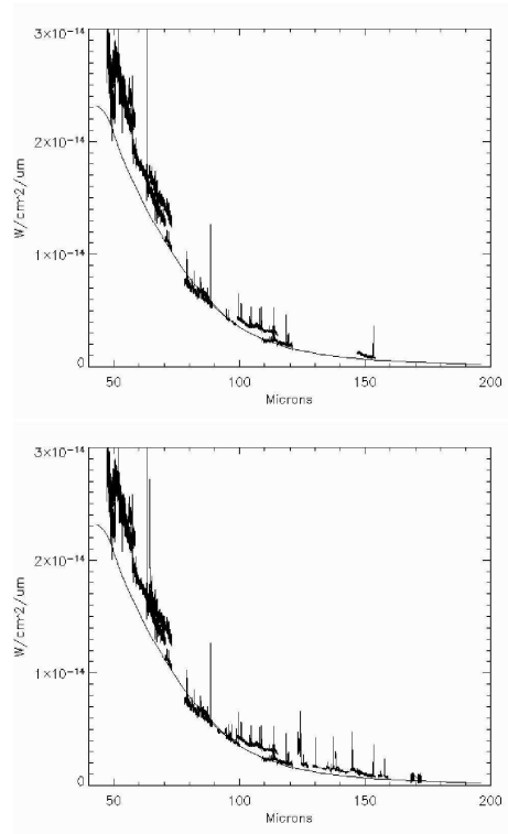
Figure 3. All L03 prime observations (upper plot) and non-prime observations (down plot) together with a continuum fit to the grating observations. Note that for wavelengths \geq 120 \mu m the spectrum is mainly covered by non-prime data.
