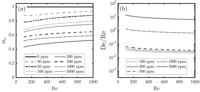
FIGURE 5. Variation in the effective flow index, found using equation 2.3 and the Carreau parameters listed in table 1 (a) and the elasticity for each fluid (b). Fluids for which the relaxation time was very small ( \lambda_r \ll 0.063 s) are omitted from (b).
