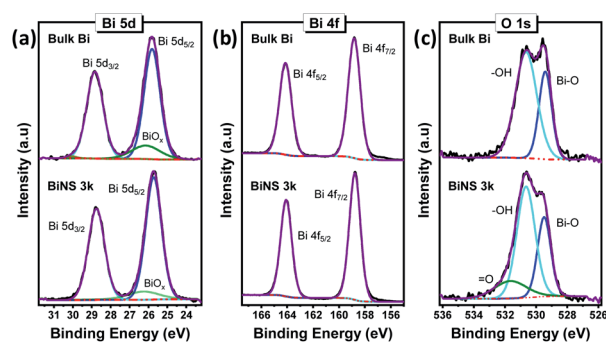
Fig. 3 High resolution XPS spectra of bulk Bi (top) and bismuthene nanosheets (BiNS 3k, bottom plots): (a) Bi 5d, (b) Bi 4f and (c) O 1s spectra.
