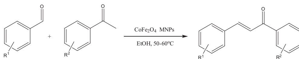
Figure 4 Aldol condensation reaction in the presence of \text{CoFe}_2\text{O}_4 MNPs.
