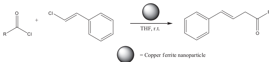
Figure 7 Synthesis of \beta,\gamma -unsaturated ketone using cinnamyl chlorides. R = (a) C 6 H 5 , (b) 2-ClC 6 H 4 , (c) furanyl, (d) -CH(CH 3 ) 2 .
