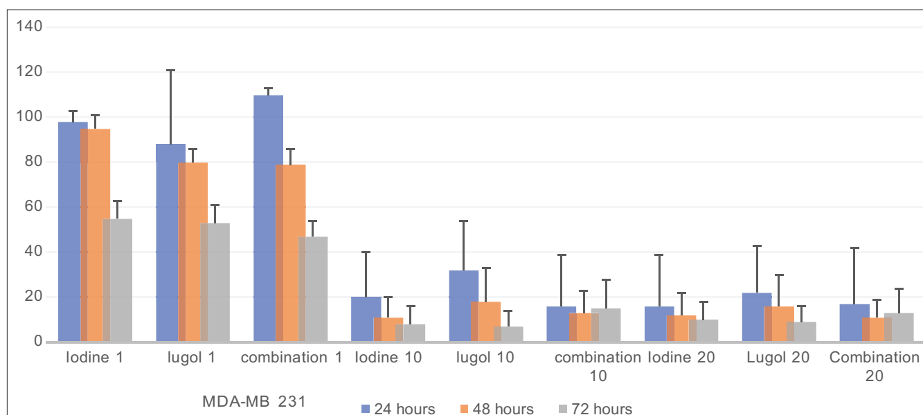
Figure 1: MDA-MB 231 cell proliferation rate of various treatments of iodine, Lugol, and combination of both for 24, 48, and 72 h. The proliferation rates reduced significantly with treatments 10 \mu M and 20 \mu M compared to 1 \mu M ( p = 0.001 , p = 0.001 , and p = 0.001 ), respectively.
