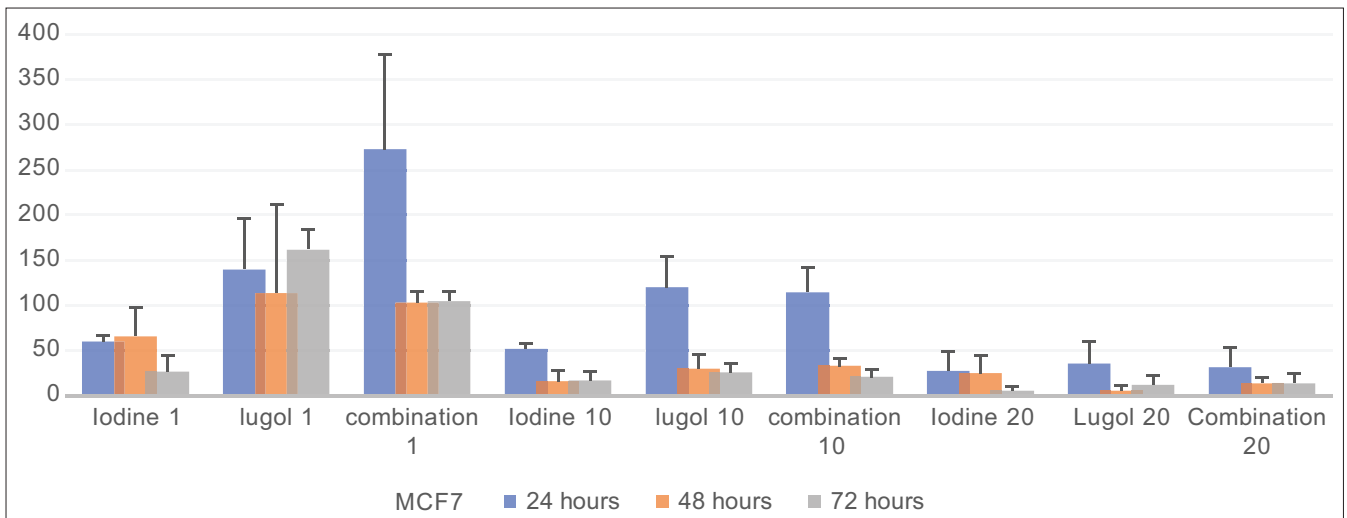
Figure 2: MCF7 cell proliferation rate of various iodine, Lugol treatments, and a combination of both for 24, 48, and 72 h. Iodine treatment doses reduced cell proliferation did not depend on the dose. Lugol and a combination of I 2 and I 3 K (10 μM) showed an antiproliferative effect after 48 and 72 h of treatments p = 0.010 and p = 0.001, respectively
