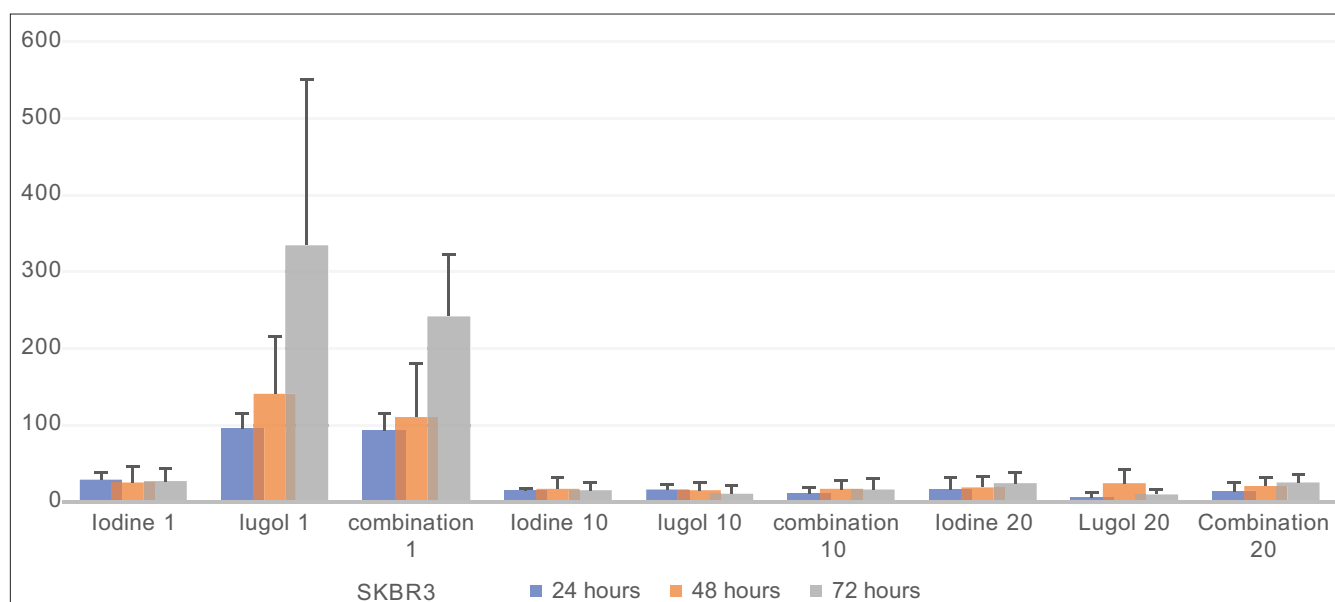
Figure 3: SKBR3 cell proliferation rate of the various treatment doses of iodine, Lugol, and a I_2 - I_3K combination for 24, 48, and 72 h. Iodine reduced the cell proliferation did not depend on the dose. Lugol and combination iodine and Lugol showed reduced cell proliferation with 10 \mu M and 20 \mu M with p = 0.001 and p = 0.001 , respectively
