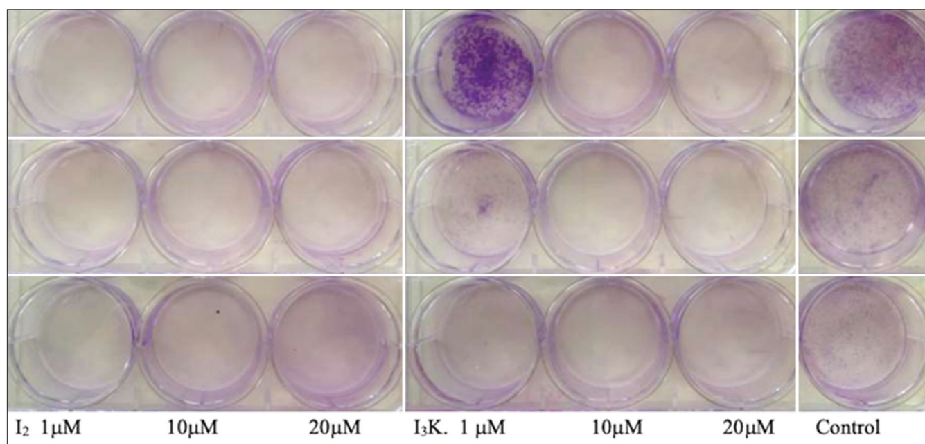
Figure 4: Clonogenic assay results, as shown on MCF7 (top), MDA-MB231 (middle), and SKBR3 (below). From left to right are results of the clonogenic assay of 1, 10, and 20 \mu M of I_2 and I_3K and control cells. I_2 suppresses cell proliferation in all doses, and the same effect showed in 10 \mu M and 20 \mu M of I_3K
