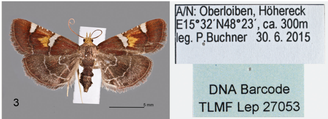
Figure 3. Pyralis regalis ([Denis & Schiffermüller]), neotype, ♂, habitus.
